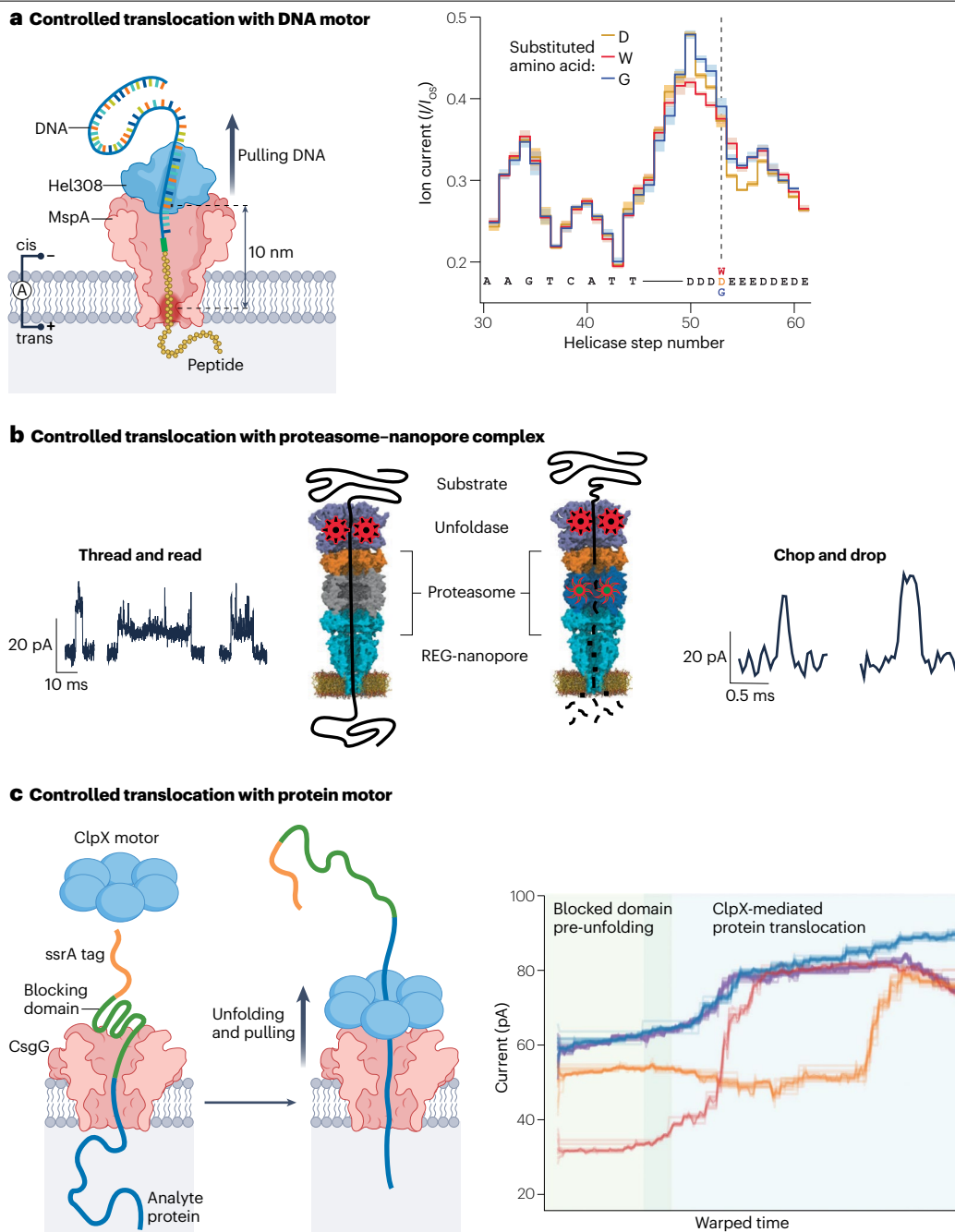
Fig. 4 | Motor enzymes can control protein translocation speed. a , Controlled peptide translocation through an Mycobacterium smegmatis porin A (MspA) nanopore can be achieved using the DNA motor enzyme Hel308. As this helicase walks along DNA, it pulls the peptide through the nanopore. The circled A at bottom left indicates applied voltage. The graph shows consensus patterns of the ion current ratio of the blocked state and open state ( I/I_{OS} ) of three DNA-peptide variants with a single amino acid substitution (D, W, G), showing identical ion current signals at the DNA section and noticeable deviation within the variant site (dashed line) 49 . b , Engineered protein complex consisting of an inactive or an active proteasome fused with an IIS regulator (REG) nanopore and a detachable unfoldase. In the ‘thread and read’ mode, full proteins containing an ssrA recognition tag are unfolded and translocated, resulting in 10–100
