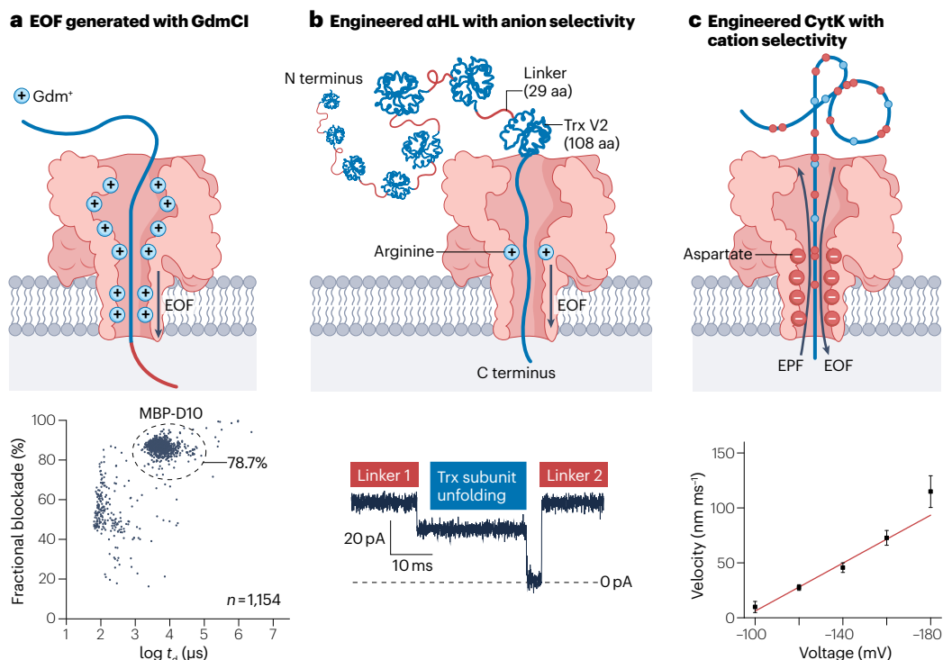
Fig. 3 | Strategies to introduce electro-osmotic flow in nanopores. a , An electro-osmotic flow (EOF) can be generated in an \alpha -hemolysin ( \alpha HL) nanopore using guanidinium chloride (GdmCl). Guanidinium ( \text{Gdm}^+ ) ions cover the vestibule of the pore and the end of the stem as 'sticky ions'. The resulting EOF and denaturing conditions allow the translocation of heterogeneously charged unfolded proteins. The scatter plot shows the protein-dependent blockade level versus the dwell time ( t_d ), in microseconds ( \mu\text{s} ), of maltose-binding protein conjugated with ten aspartate residues (MBP-D10) 46 . b , By mutating the constriction site in an \alpha HL nanopore with positively charged arginine, an EOF can be generated to unfold and translocate mixed-charged thioredoxin
