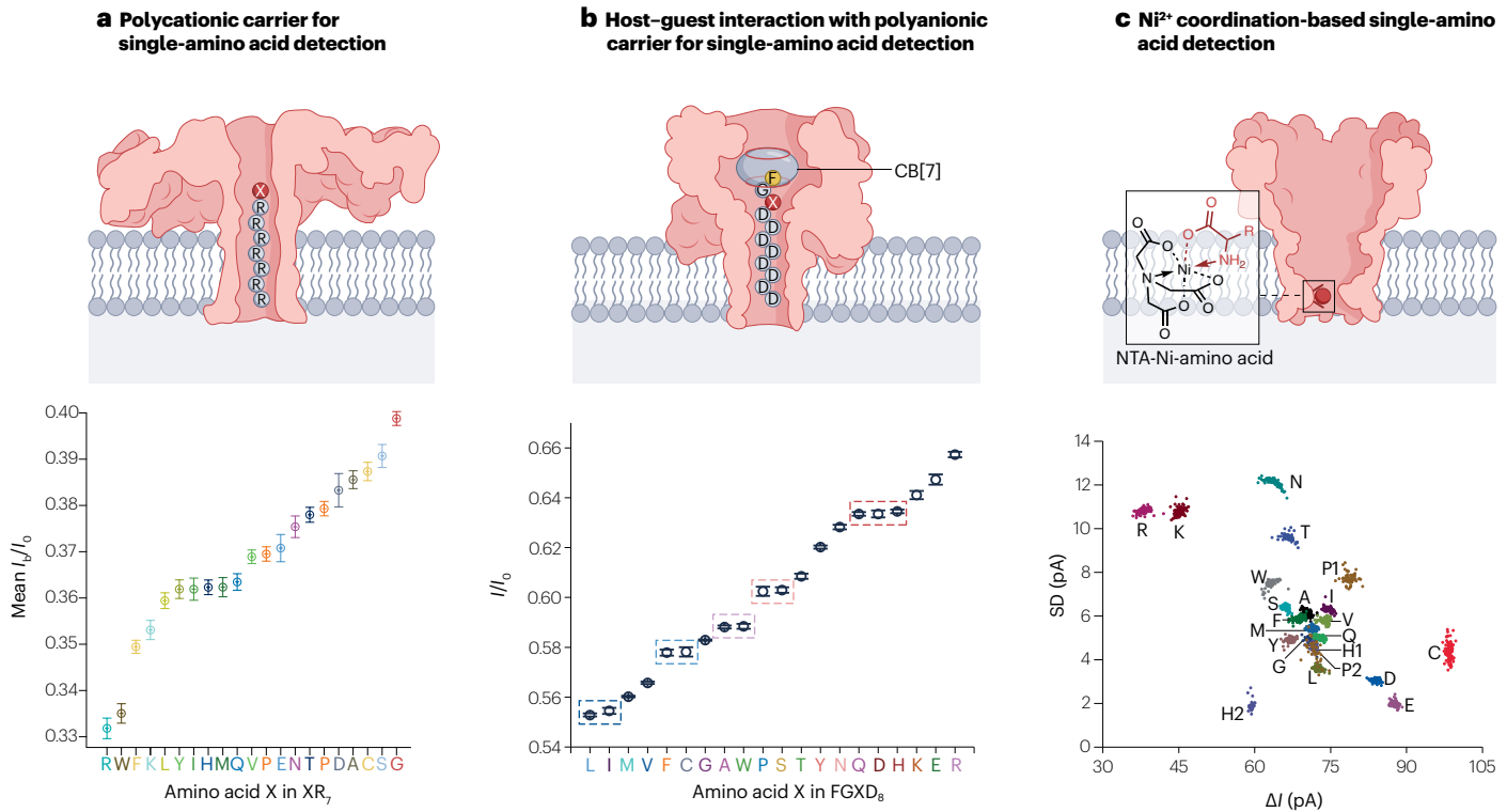
Fig. 2 | Single amino acids can be discriminated using nanopores. a, Amino acids connected to a polycationic carrier can be inserted into a wild-type aerolysin nanopore. The mean I_b/I_o (ratio of the ionic current ( I_b ) when a molecule is inside the pore to the open-pore current ( I_o ) in an empty nanopore) values of all 20 amino acids can be measured with this system 67 . b, In an \alpha -hemolysin ( \alpha HL) nanopore, an amino acid connected to a polyanionic carrier engages in a host-guest interaction with cucurbit[7]uril (CB[7]) at the constriction
