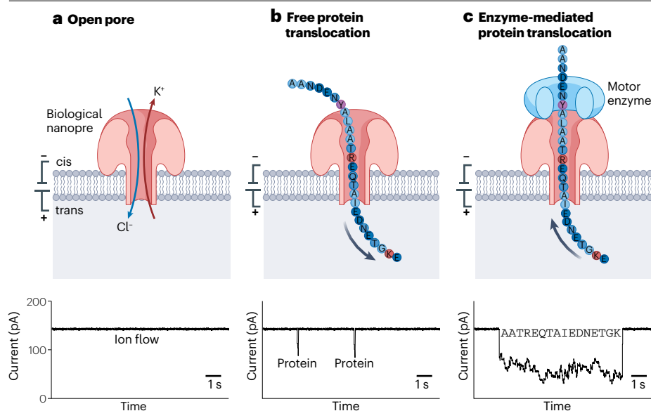
Fig. 1 | Nanopore-based protein sequencing. a , A biological nanopore is inserted in a synthetic or biological membrane that separates two electrolyte compartments. A voltage is applied across the membrane, causing an active ion flow through the nanopore. b , Protein translocations result in sudden ion current dips as proteins pass through the pore. c , A motor enzyme capable of walking on the protein strand slows down protein movement through the pore, resulting in a longer-duration signal with distinct ion-current changes, which can be assigned to specific parts of the protein sequence.
