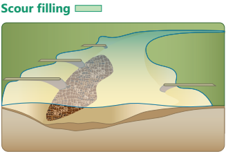
Material: sediment of 4-150 mm
