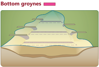
Material: boulders of 60-300 kg
