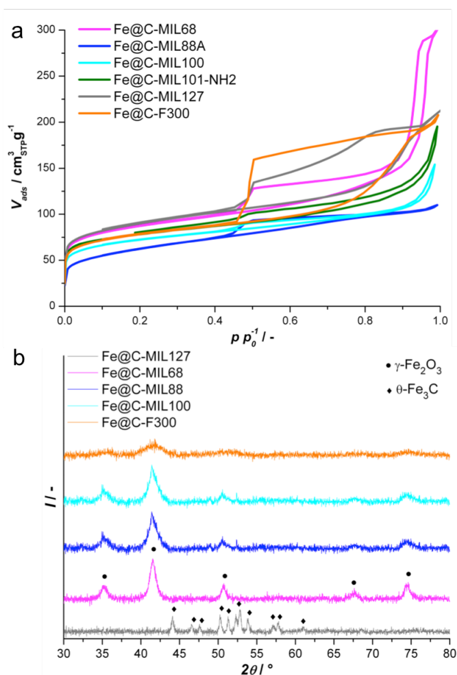
Figure 2. a) Nitrogen uptake at 77 K per gram of Fe@C catalyst and b) XRD of the Fe@C catalysts, indicating the presence of nanosized \gamma\text{-Fe}_2\text{O}_3 and \theta\text{-Fe}_3\text{C} phases present after passivation.
