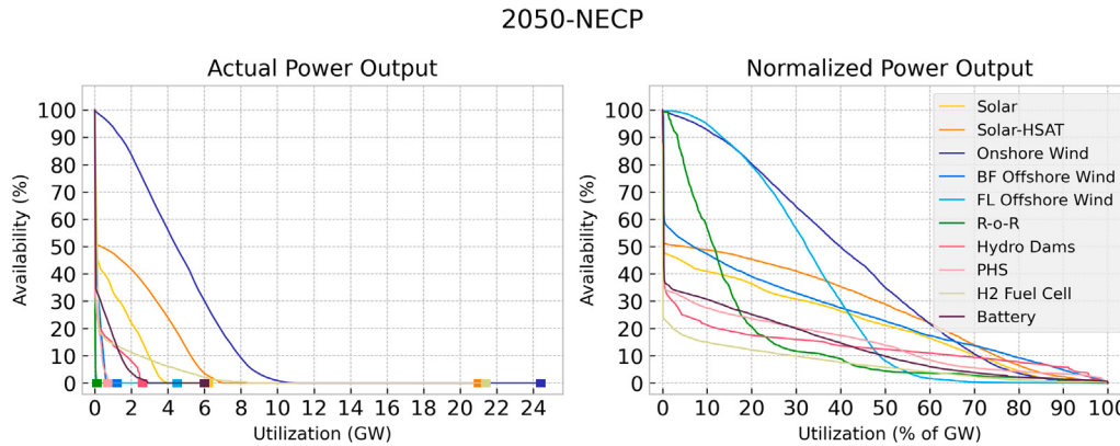
Fig. 12. Survival function of power output for generators and storage units for 2050 NECP scenario. Right figure represents the function with a normalized x-axis for all generators (% of GW), and left figure shows their actual power output for the corresponding amount (%) of time-steps (availability).
