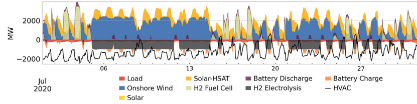
Fig. 7. Time-series of a bus in Thrace for 2050, with large capacity of H 2 electrolyzers and fuel cells.
