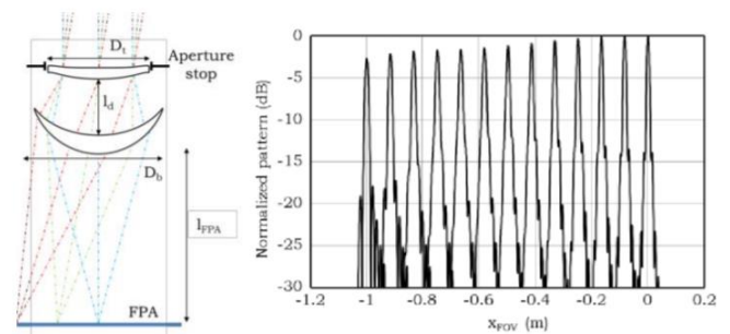
Fig. 1. Flipped dual-lens design: (a) geometry, (b) simulated beams at 500GHz
