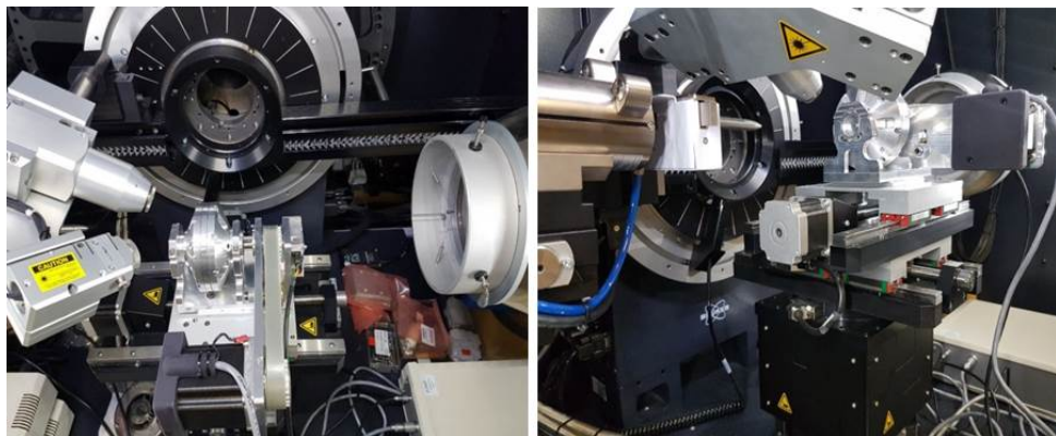
Figure 3.12: An image of the developed Couette shear cell mounted at the lab-scale X-ray diffractometer Bruker D8-Discover
