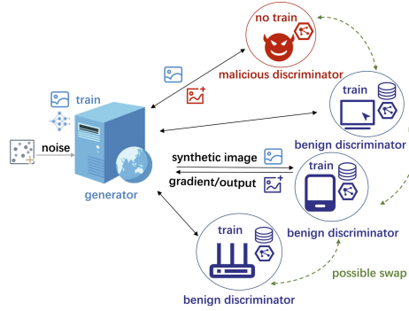
Fig. 1. Architecture of Multi-Discriminator GAN: one generator, and four discriminators, one of which being free-rider.
