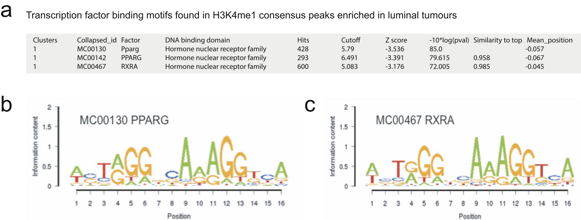
Figure 4. Functional analysis of H3K4me1-marked enhancers. (a) Differential H3K4me1 consensus peaks were analysed for enrichment of transcription factor binding motifs. Shown are the motifs that are enriched in the luminal tumours. (b) The PPARG consensus motif identified in the motif search. (c) The RXRA consensus motif identified in the motif search.
