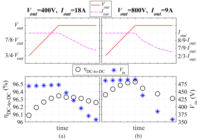
Fig. 16. Measured \eta_{dc-to-dc} and used V_{in} during a typical battery charging profile with the CC and the CV modes at aligned BPPs while the V/I -D converter operates as (a) current doubler and (b) voltage doubler. These results summarize that the V/I -D converter is a universal solution for charging 400- and 800-V EV batteries efficiently at the same power.
