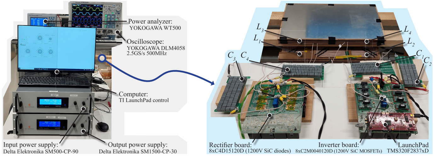
Fig. 9. Equipment and implemented 7.7-kW laboratory prototype of the V/I -D converter employing coupled BPPs.
