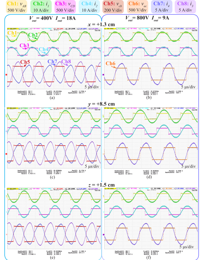
Fig. 15. Measured circuit waveforms at the nominal V_{out} and rated P_{out} when the V/I -D converter operates with misaligned BPPs as (a), (c), and (e) current doubler ( V_{out} = 400\text{V} ) and (b), (d), and (f) voltage doubler ( V_{out} = 800\text{V} ). The misalignment is (a) and (b) x = 1.3\text{cm} , (c) and (d) y = 8.5\text{cm} , and (e) and (f) z = 1.5\text{cm} . The misalignment is performed only with respect to one axis at a time.
