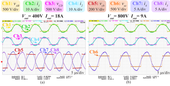
Fig. 14. Measured circuit waveforms at the nominal V_{out} and rated P_{out} when the V/I -D converter operates with aligned BPPs as (a) current doubler ( V_{out} = 400\text{V} ) and (b) voltage doubler ( V_{out} = 800\text{V} ).
