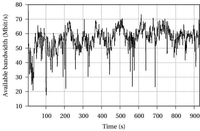
Fig. 3: Available bandwidth on a 100 Mbps WAN link [15].
