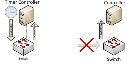
(a) While a flow is active, the controller can - f.e. using a timer or other event - query the switch to retrieve flow specific statistics. (b) The end of a flow is announced by sending a FlowRemoved packet to the controller.
