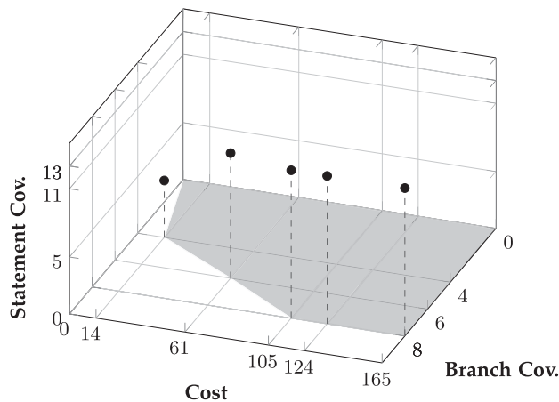
(a) Branch Coverage
