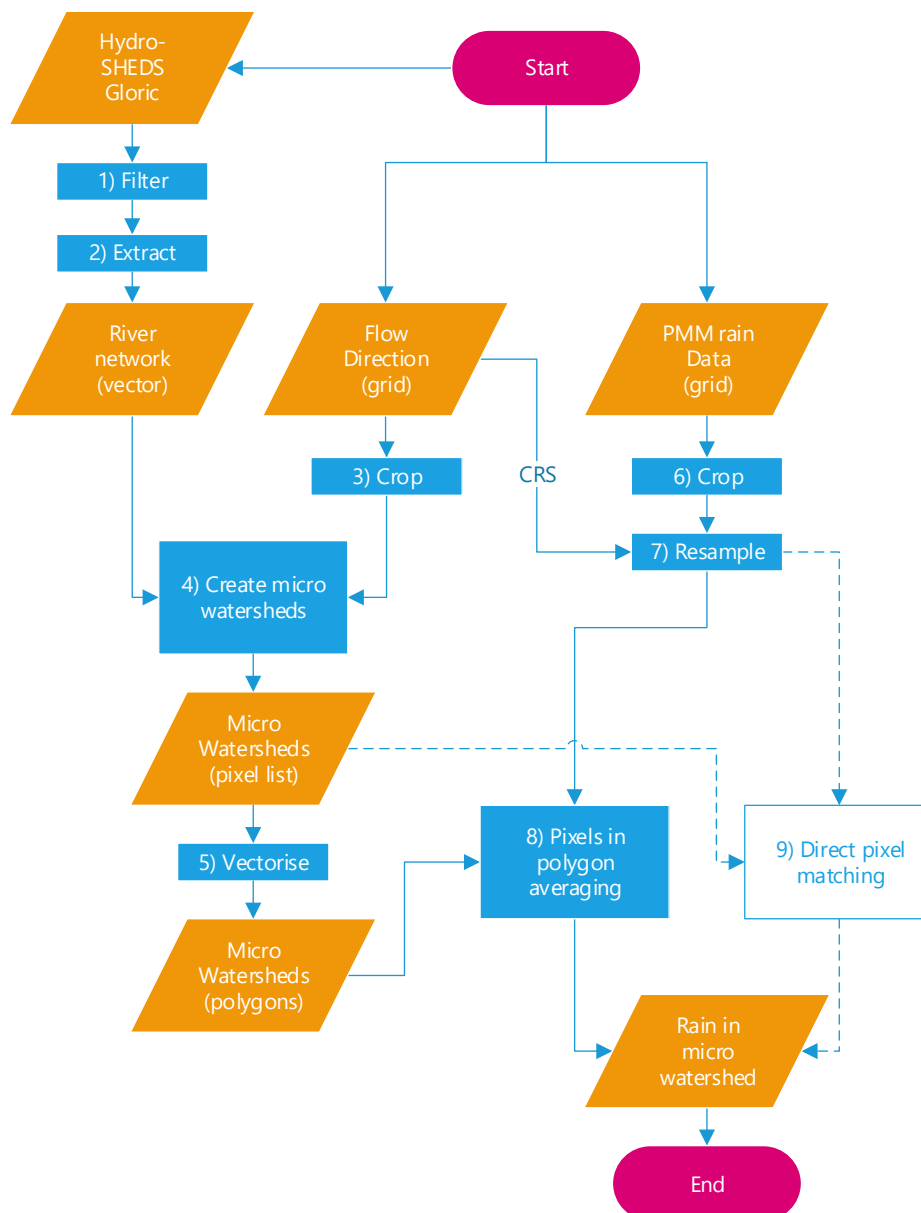
Figure B.4: Schematic showing all steps taken in data processing. Blue blocks are processing steps and orange blocks are datasets. The processing steps corresponds to the file main_data.py .
