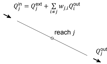
Figure 4.2: Schematic displaying a single reach represented as an edge with its inflow and outflow. For weighting factors 0 \geq w_{j,i} \leq 1 holds. These are typically zero except for the connected reaches. Note that \sum_j w_{j,i} = 1 for all reaches i .
