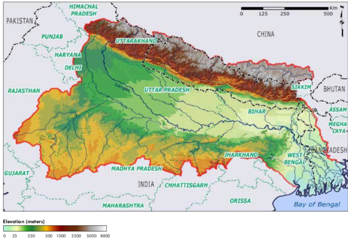
Figure 6.1: The elevation map of the Ganges basin. The Ganges rises in the Himalaya and within 200 kilometres the landscape changes from mountainous to the flat Ganges plains. The river ends in a flat delta and flows through the earth's largest mangrove ecosystem. (World Bank, 2014)
