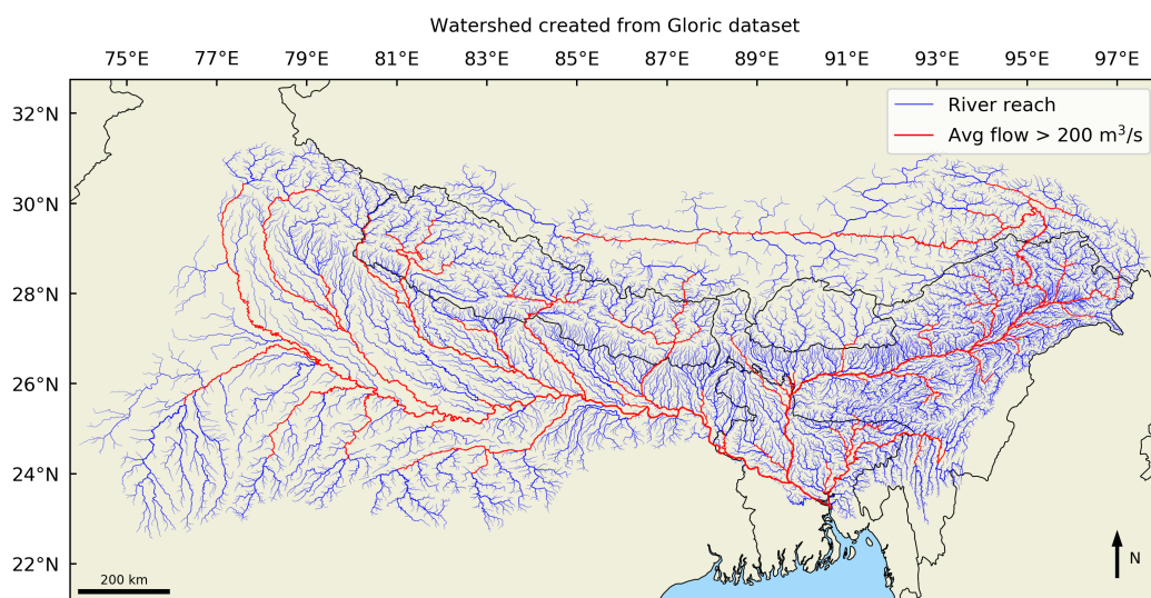
Figure 6.4: Figure showing the reaches extracted from the GloRIC dataset. When compared to figure 6.2 the main tributaries are in close agreement. One notable difference is that the HydroSHEDS dataset does not contain bifurcations. This can be seen, for example, in the delta where the Hooghly river is missing that flows through Kolkata.
