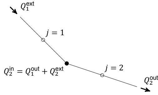
Figure 4.4: Two reaches represented as two connected edges in a network: the inflow of reach 2 is defined as the outflow of reach 1 plus an external inflow Q_2^{\text{ext}} . The external inflow can be any other source of water flowing in or out of this reach. Examples are: precipitation, ground water flow or surface water run-off.
