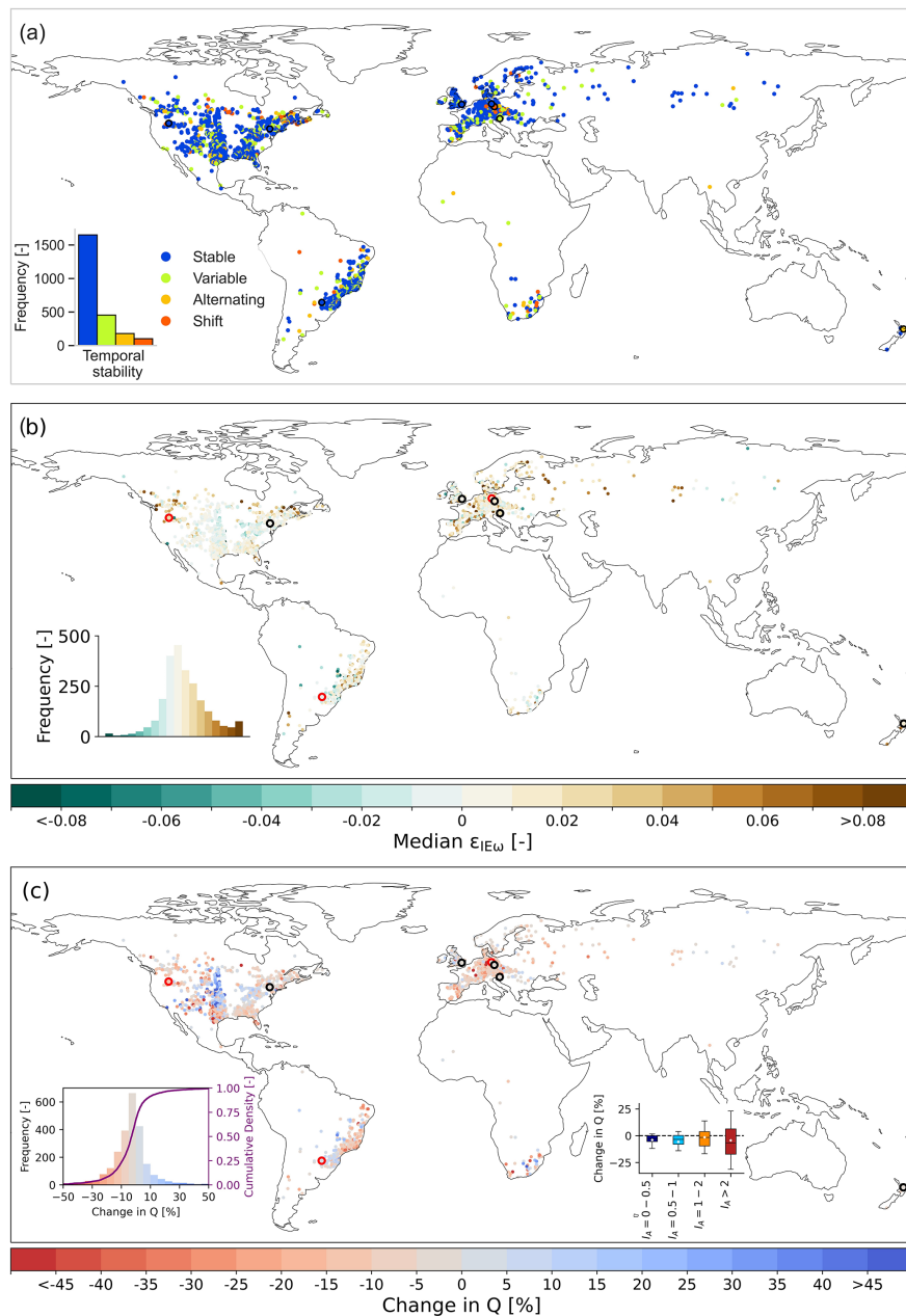
Figure 7. (a) Temporal stability and (b) long-term median \varepsilon_{IE\omega} value maps of aggregated long-term marginal distributions for the study catchments and (c) change in Q as a result of long-term median \varepsilon_{IE\omega} values. Histogram and cumulative density of change in Q and change in Q across different I_A bins are presented as two insets. Change in Q reflects the change due to median deviation \varepsilon_{IE\omega} values from the expected parametric Budyko curve only (i.e. excluding any change resulting from a change in aridity and its associated movement along the expected curve). Catchments highlighted with a black border represent the five selected examples from Fig. 6, while those outlined in red denote three additional selected example catchments shown in the Supplement (Fig. S5). The boxes represent the 25th to 75th percentiles, while whiskers extend to the 10th and 90th percentiles. Diamonds denote the arithmetic mean, and outliers are not shown.
