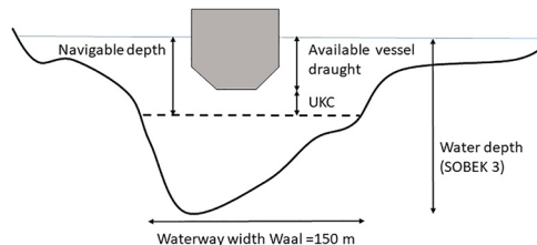
Fig. 3. Link between water depth and available vessel draught.
