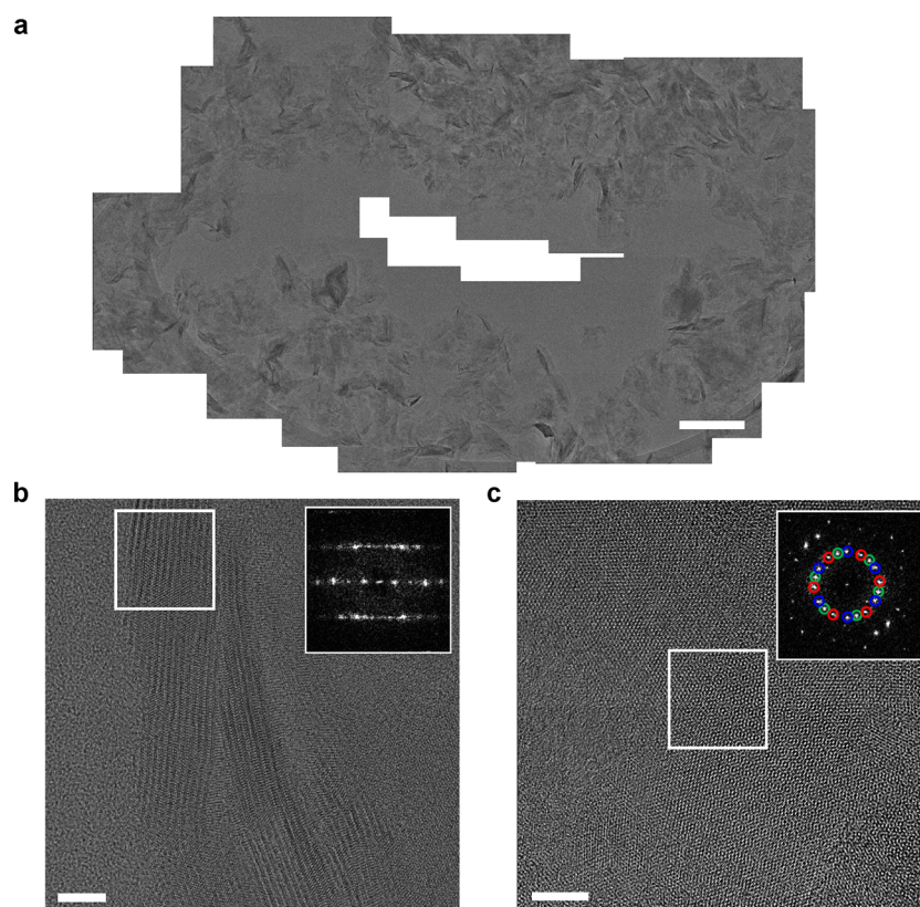
Figure 5. (a) Low-magnification TEM image of a MoS 2 patch aligned in the in-plane direction. (b) HRTEM image of vertically aligned MoS 2 nanosheets along the [1120] direction with its corresponding FFT calculated in the area marked by a white square as the inset. (c) HRTEM image of a Moiré region in MoS 2 , where the FFT in the inset displays the overlap of three MoS 2 nanosheets along the [001] direction. The scale bar in part a corresponds to 200 nm; those in parts b and d correspond to 5 nm.
