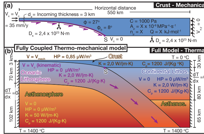
FIGURE 2 Model setup. Model setup, with the specification of thermal and mechanical parameters. S is the point where the subducting plate contacts the Moho of the upper plate. A set of velocities, V , are defined with regards to a fixed frame in the upper-plate interior: V_x and V_y are the components of velocity in horizontal and vertical directions, respectively, and V_{mech} is the 2-D velocity in the mechanical domain and is a free variable. Boundary conditions are a constant convergence velocity, V_c , applied to the left side, and the base of the subducting plate. Boundary between slab and upper plate has a frictional failure criterion, by which relative slip occurs on the boundary once the criterion is exceeded. The incoming sediments have a thickness of d_a . D_s is the flexural rigidity of the subducting plate and D_o is that of the overriding plate. The internal friction angle is shown as \phi , and the friction angle between plates is \phi_b . A_\mu is the coefficient of the power-law viscosity and n_\mu is its coefficient, with Q being the activation energy. HP = heat production, K = thermal conductivity, C_p = specific heat, C = cohesion and T = temperature. Material deforms viscously until yield stress is exceeded, at which point it deforms to satisfy the yield criterion
