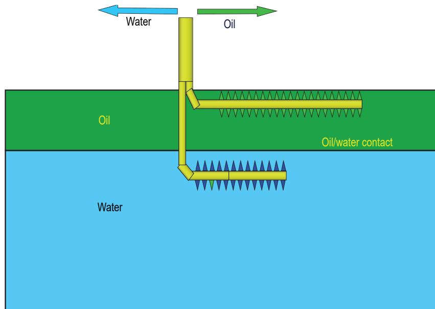
Figure 1.4: Schematic presentation of BWS production [64].
