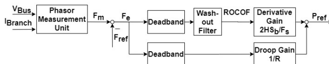
Fig. 10. Diagram of droop and derivative control.
