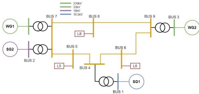
Fig. 7. IEEE 9 bus system with 52% wind generations.
