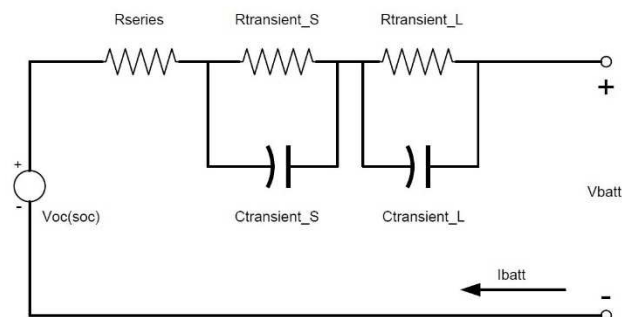
Fig. 11. Structure of battery model.
