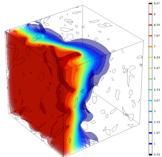
Figure 5. Iso-surface of electric potential (units in V)
