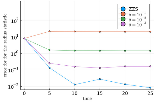
(b) Error for the radius for the ZZS and its approximations given by Algorithm 2.
