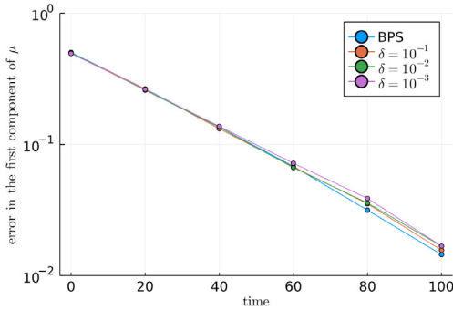
(c) Error for the mean for the BPS and its approximations given by Algorithm 3.
