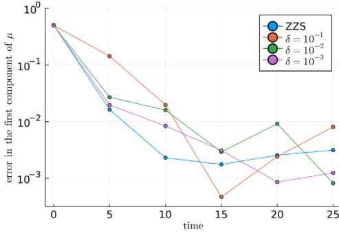
(a) Error for the mean for the ZZS and its approximations given by Algorithm 2.
