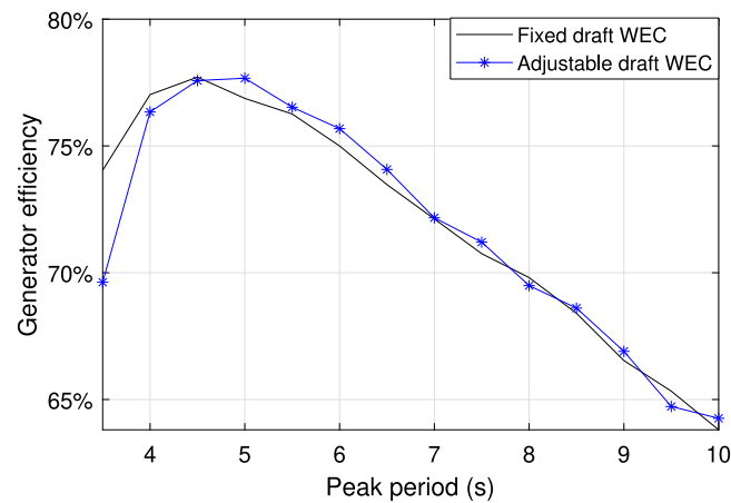
Fig. 23. Comparison between the generator efficiency of the adjustable draft WEC and of the fixed draft WEC, with H_s = 2.5 m and \sigma_F = 40 kN.
