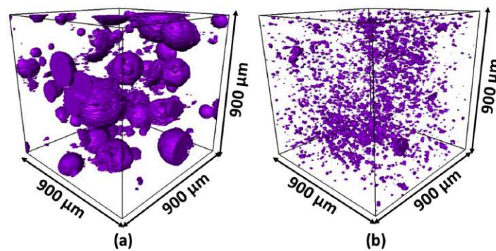
Figure 7. X-ray computed tomography scans showing distribution of two types of PCM microcapsules in cement paste: (a) PCM-A (agglomerated microcapsules, see Figure 6); and (b) PCM-B (discrete particles, see Figure 6) [65].
