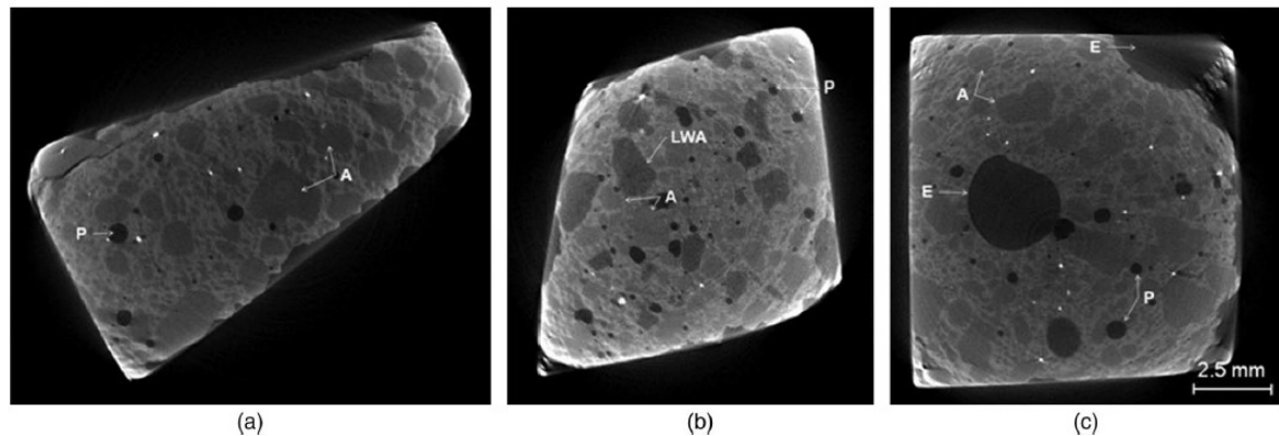
Figure 4. Microtomographs of investigated mortars: (a) control mortar without PCM, in which quartz aggregate (A) and pores/air voids (P) are easily visible; (b) mortar containing lightweight aggregate (LWA)-PCM, which appears similar to quartz aggregate but darker because of its lower density; and (c) mortar containing encapsulated PCM pellets (E) [43].
