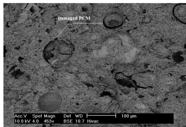
Figure 9. SEM micrograph (using back-scattered electron (BSE) detector) of concrete fracture surface showing damaged or collapsed PCM particles still occupying their original void [75].
