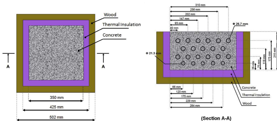
Figure 15. Design details for the large-scale concrete slab: (left) top view details of the mold and the concrete slab; (right) cross section details of the mold and the concrete slab with embedded pipes (to prevent heat transfer through metal pipes, additional outer thermal insulations were installed on both sides of the framework where pipes were out of the wood framework) [32].
