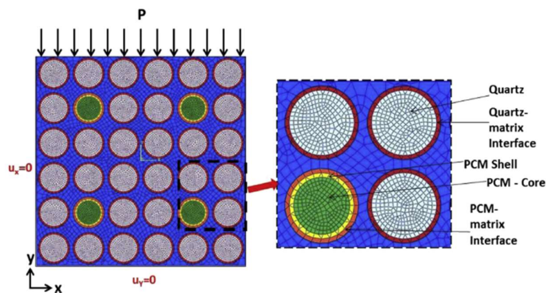
Figure 23. Finite element (FE) model showing the boundary conditions, applied compressive loading, and a magnified representation of the inclusions with the zones around them. The model contains 50% of inclusions (mortar with 10% PCM-E particles replacing quartz particles) by volume (or area) [65].
