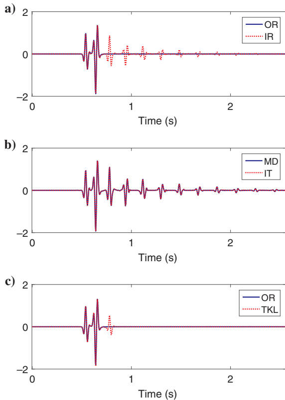
Figure 4. (a) A comparison of non-zero-offset (800 m) traces from the original and retrieved data sets shown in Figure 2a and 2b, (b) a comparison of non-zero-offset (800 m) traces from the modeled primary reflections and retrieved data sets shown in Figure 2e and 2c, and (c) a comparison of non-zero-offset (800 m) traces from the original and retrieved data sets shown in Figure 2a and 2d.
