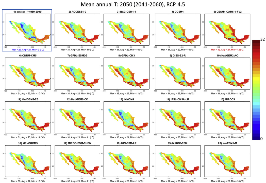
FIGURE 3.11 Spatial distribution of mean annual T (°C) over Mexico for the period 2041–60 (2050): baseline and 19 GCMs, and RCP 4.5. GCM , General Circulation Model; RCP , Representative Concentration Pathway; T , temperature.
