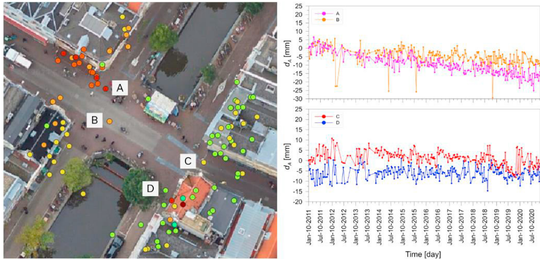
Fig. 3. LOS deformation of PSs detected in the proximity of the abutments of Bridge 215 in ascending geometry.
