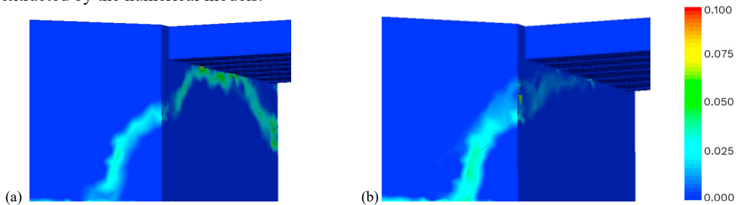
Fig. 6. Principal tensile strains of the analysed scenario for a max vertical displacement equal to 10 mm: symmetric (a) and asymmetric (b) configuration.
