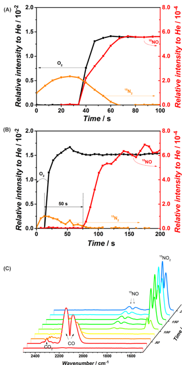
Figure 1. 15 NO, 15 N 2 , and O 2 evolution upon 0.2 % 15 NO + 5% O 2 exposure over reduced Rh/ceria (A) at 600°C with space velocity at 125.000 l/h, (B) at 450 °C with GHSV of 67.000 l/h; (C) FT-IR spectral responses of (B).
