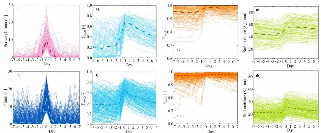
Figure 4. Sensitivity analysis of variability of the young water fractions (<3 months) in river flow ( F_{wy,Q} ) and evaporation ( F_{wy,E} ) as well as soil moisture S_u in response to the selected snowmelt events in winter in (a)–(d) and rainfall events in summer in (e)–(h).
