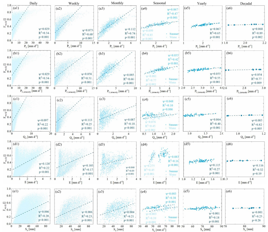
Figure 3. Relationship between the young water fraction in river flow ( F_{wy,Q} ) and hydro-climatic variables over different time scales from daily to decadal including (a) liquid precipitation P_L (rainfall + snowmelt), (b) liquid precipitation intensity P_{L,intensity} , (c) river flow Q_o , (d) evaporation E (e) soil moisture S_u . The dashed lines indicate the linear relationships between the F_{wy,Q} and the various hydro-climatic variables x , used to approximate the sensitivity \psi = \Delta F_{wy,Q} / \Delta x .
