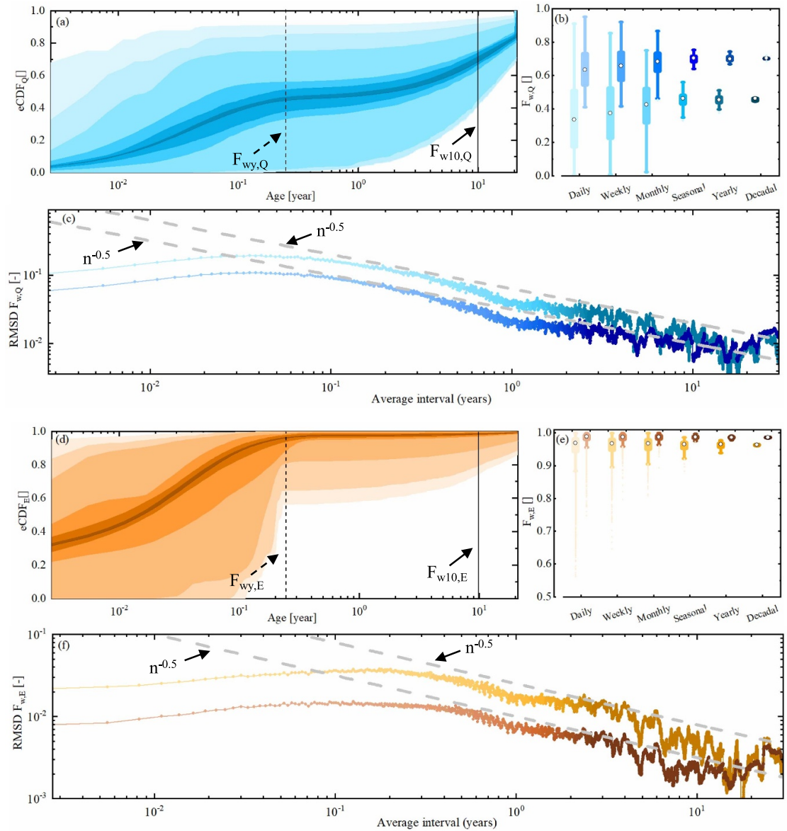
Figure 2. The variability of river flow TTDs (eCDF Q ) and evaporation TTDs (eCDF E ) from the most balanced model solution over various time scales. (a) The blue shades from lighter to darker indicate the 5th/95th intervals of the eCDF Q of the river water age distributions from daily to decadal averaging time-scales, (b) the blue and navy blue box plots (whiskers indicate 5th/95th percentiles) from lighter to darker indicates F_{wy,Q} and F_{w10,Q} from daily to decadal, respectively, (c) Root mean squared differences (RMSD) between pairs of successive average values in F_{wy,Q} (the gradient blue line) and F_{w10,Q} (the gradient navy blue line) plotted against corresponding averaging intervals, (d) the orange shades from lighter to darker indicate the eCDF E of the evaporation water age distributions from daily to decadal, (e) the yellow and brown boxes from lighter to darker indicates F_{wy,E} and F_{w10,E} from daily to decadal, respectively, (f) RMSD in F_{wy,E} (the gradient yellow line) and F_{w10,E} (the gradient brown line). Note that the dashed grey line is the slope of -0.5 predicted by the central limit theorem for self-averaging time series and n is the number of averaging time steps (here: years).
