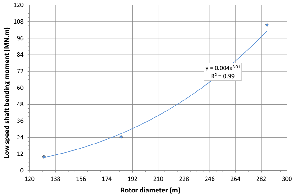
Figure 5: Upscaling of low speed shaft bending moment from 5 to 20 MW reflecting the increase of gravity loads using the optimized wind turbine data
