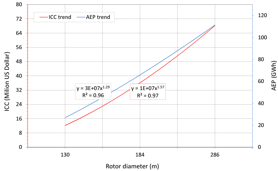
Figure 16: ICC and AEP trade-off for upscaled wind turbines from 5 to 20 MW shows how upscaling impacts the costs.
