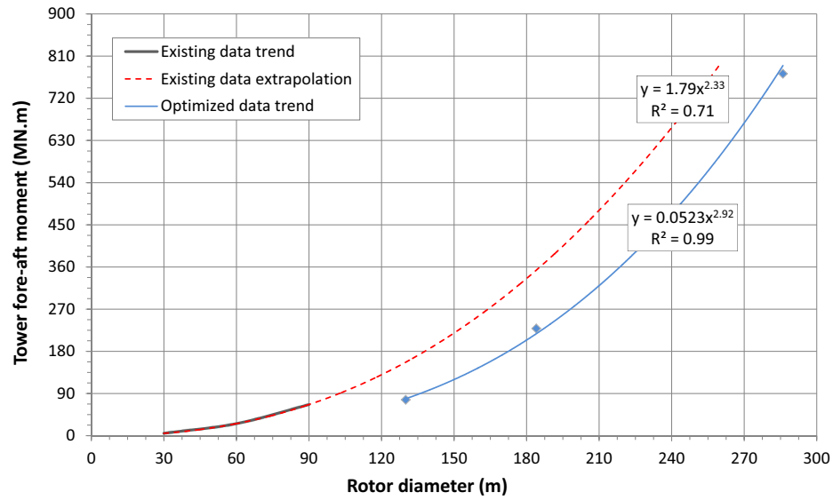
Figure 7: Upscaling of the tower fore-aft bending moment from 5 to 20 MW corresponding the increase of rotor thrust
