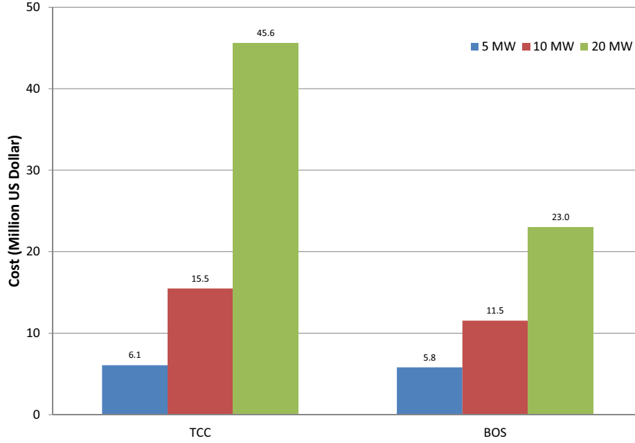
Figure 15: TCC and BOS for the optimized 5 to 20 MW wind turbines show a rapid increase in TCC
