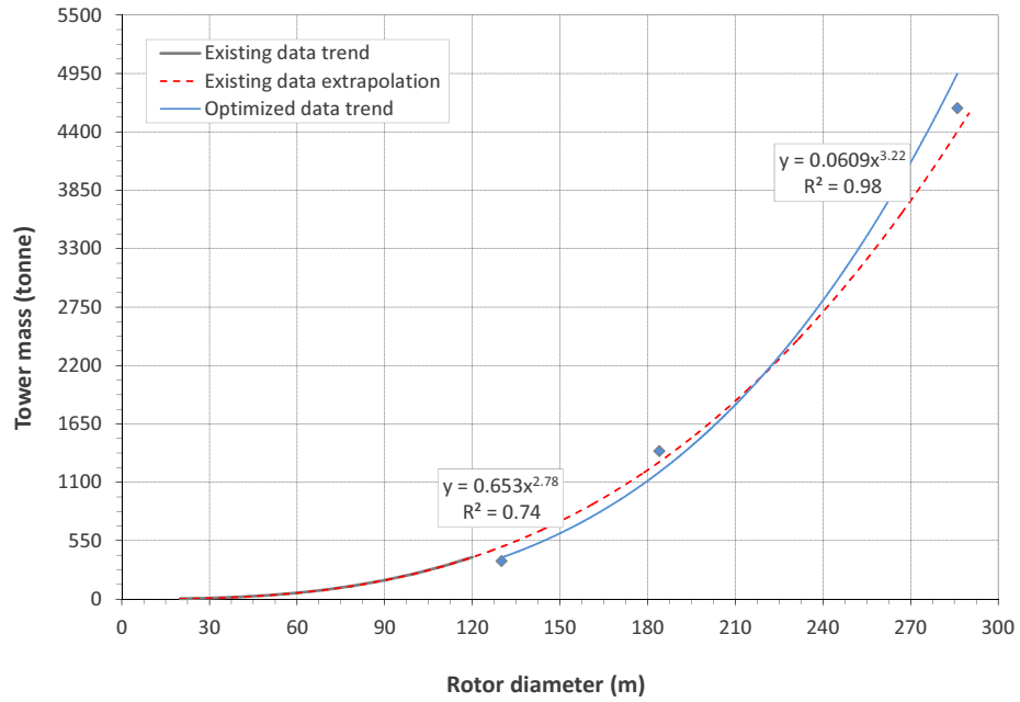
Figure 12: Upscaling of the tower mass from 5 to 20 MW showing the effect of linearly varying thickness and diameter of the optimized design
