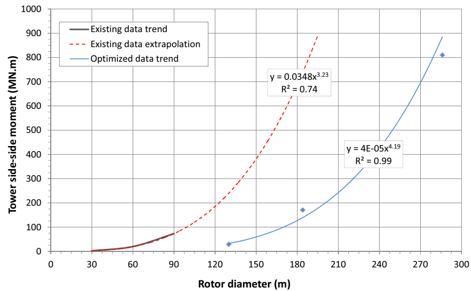
Figure 8: Upscaling of the tower side-to-side bending moment from 5 to 20 MW showing the increased dynamic amplification of loads
