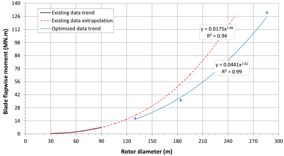
Figure 3: Upscaling of blade flapwise loads from 5 to 20 MW to show the increase of aerodynamic loads
