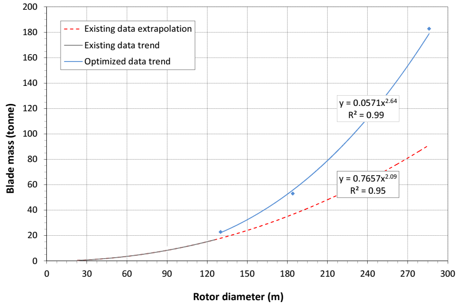
Figure 11: Scaling of a single blade mass from 5 to 20 MW showing the negative influence of upscaling
