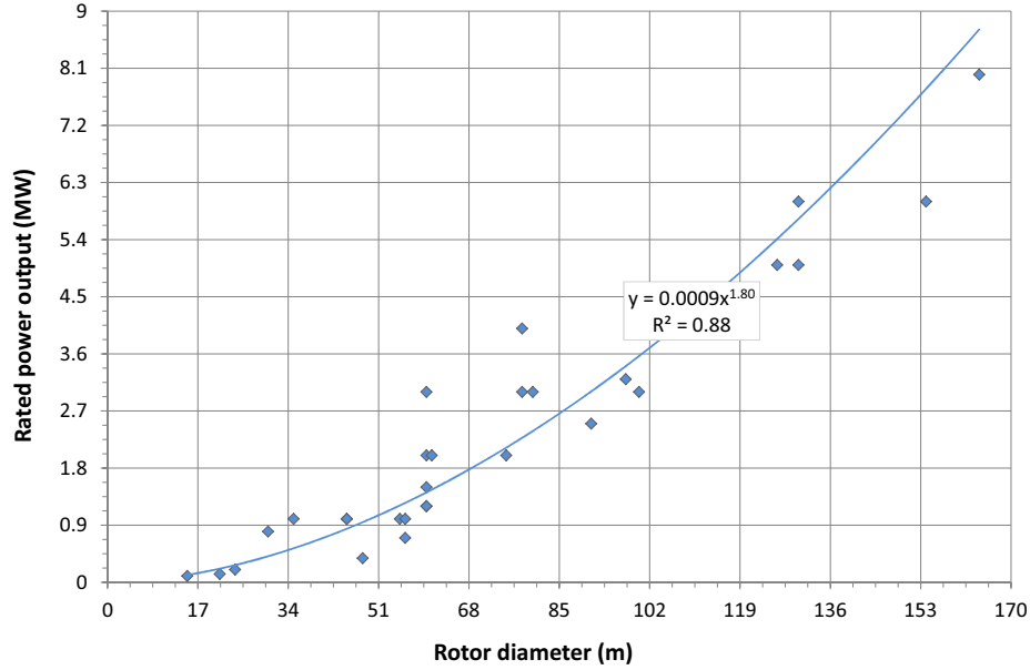
Figure 1: Rated power output of the wind turbine as a function of rotor diameter. These data are collected by the authors from public product brochures and company web sites. Professional database services also exist to buy these data collectively. 4
