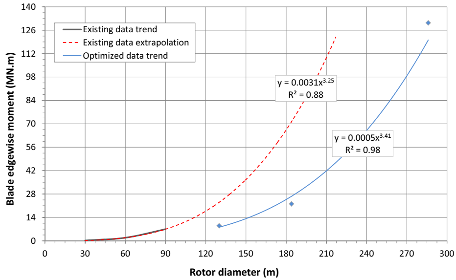
Figure 4: Upscaling of blade edgewise loads from 5 to 20 MW to show the increase of gravity loads
