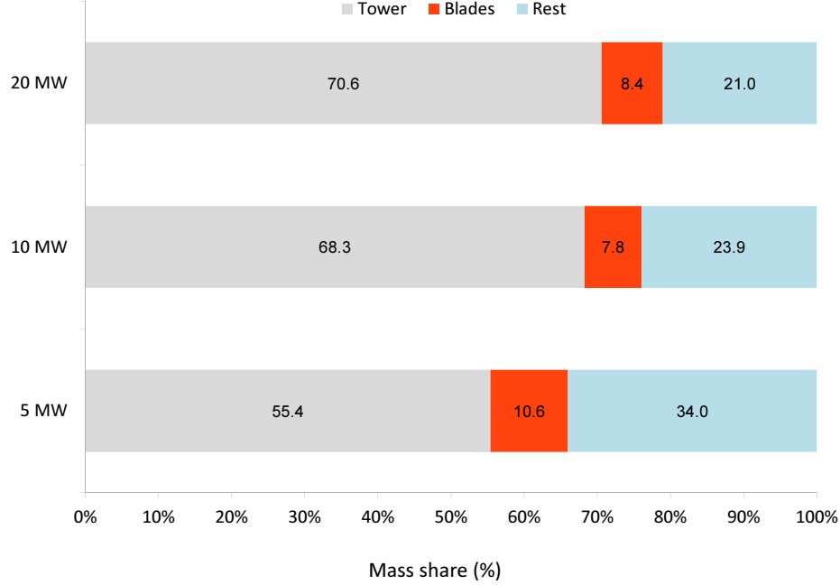
Figure 13: Mass breakdown of components from 5 to 20 MW showing how upscaling influences blade and tower mass
