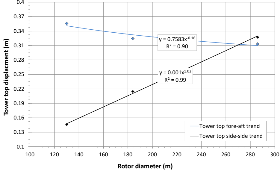
Figure 9: Upscaling of the tower top side-to-side bending motion from 5 to 20 MW showing the increased flexibility of the system
