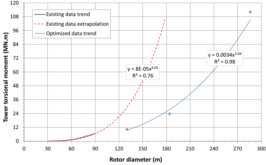
Figure 10: Upscaling of the tower torsional moment from 5 to 20 MW showing mismatch of the existing data trend with optimized and analytic scaling
