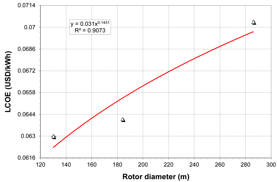
Figure 17: Trend of LCoE for wind turbines ranging from 5 to 20 MW, showing the overall negative impact of upscaling
