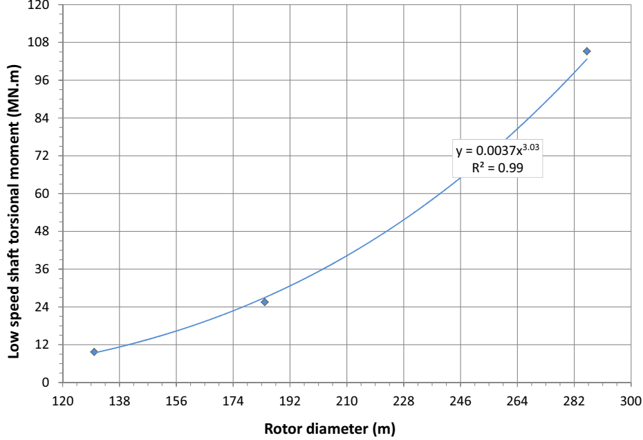
Figure 6: Upscaling of low speed shaft torsional moment from 5 to 20 MW reflecting the increase of rotor torque using the optimized wind turbine data
