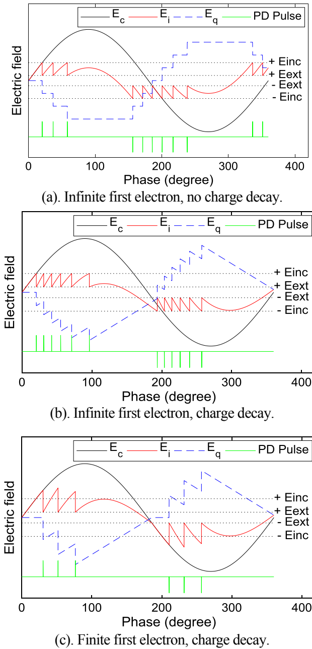
Fig. 2. Electric fields during PD.
