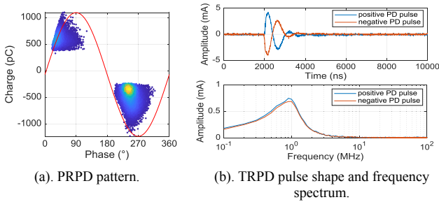
Fig. 18. Test 6: Characteristics of PD in cable sample 1.
