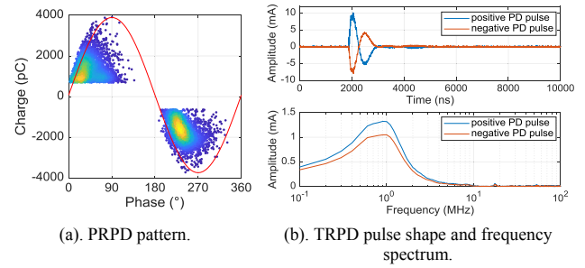
Fig. 6. Characteristics of PD type I in cable sample 1 at 17\text{ kV}_{\text{pk}} .
