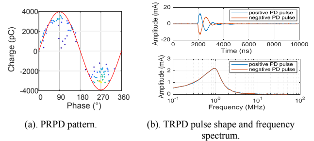
Fig. 15. Test 5: Characteristics of PD in cable sample 1.
