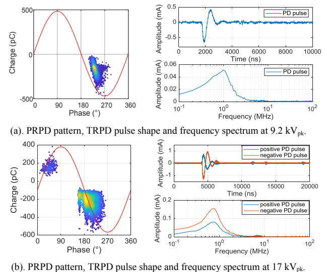
Fig. 7. Characteristics of PD type II in cable sample 2.
