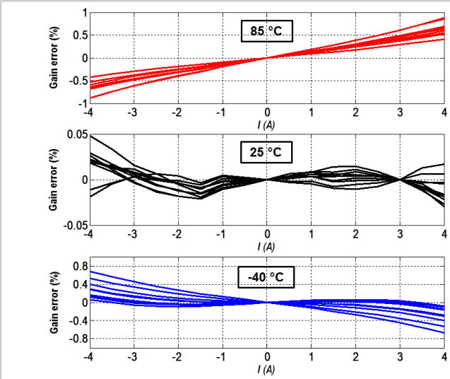
Figure 19.4.4: Measured current-sensing gain error at different ambient temperatures (10 samples).
