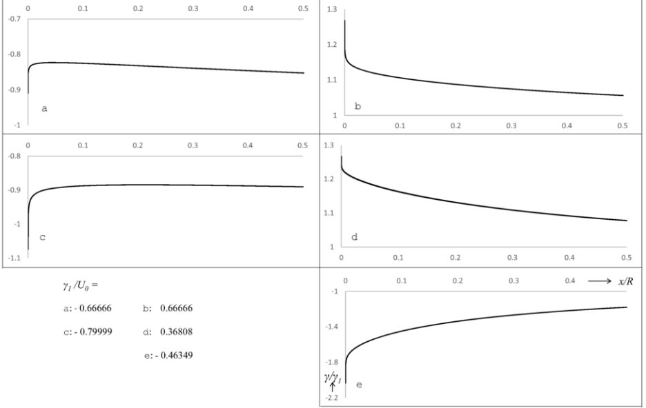
Figure 7.4. The distribution of the vortex sheet strength \gamma_\varphi(x)/|\gamma_{\varphi,1}| , for flow cases a to e, defined in table 6.1. The vertical axes have the same scale, except the axis of e, which covers a 4 times larger range of \gamma .
