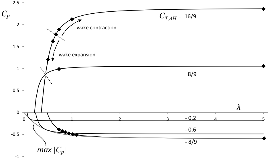
Figure 6.5. The Joukowsky momentum theory results (black lines), calculated values (♦, see section 6.4) and the maximum wind turbine |C_p| (grey line).
