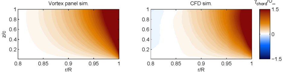
Figure 8.7. The chordwise vorticity determined by difference in radial velocities.
