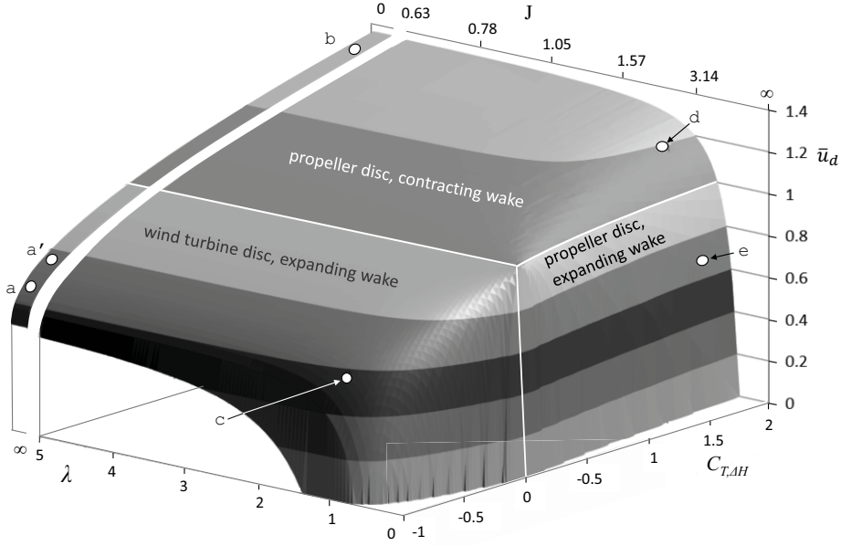
Figure 6.2. The axial velocity \bar{u}_{x,d} for discs extracting energy from the flow ( -1 < C_{T,\Delta H} \leq 0 ) and discs adding energy ( 0 \leq C_{T,\Delta H} < 2 ) for 0 \leq \lambda \leq 5 and for \lambda = \infty . The markers a' and a to e refer to flow cases defined in Table 6.1 and analysed in the next sections. Flow states a and b correspond to the flow states with the same markers in chapter 5.
