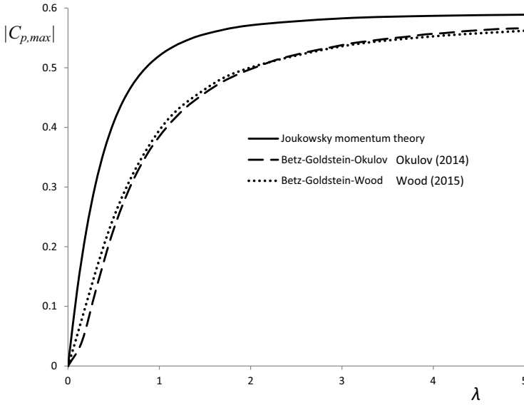
Figure 6.11. The Joukowski actuator disc |C_{p,max}| compared with the Betz-Goldstein |C_{p,max}| solutions of Okulov (2014) and Wood (2015) for rotors with an infinite number of blades.
