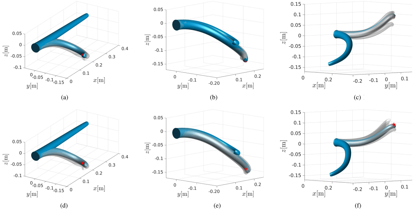
Fig. 8. Frame sequences of robot motion, divided in three time windows. Panels (a)–(c) and (d)–(f) show the robot when controlled in the y or q coordinates using the laws (24) and (25), respectively. The initial and final configurations of each interval are shown in blue while light gray shapes represent intermediate configurations. A red star indicates the constant target position of the end-effector. (a) P-satI-D in y space; t \in [0; 2] s. (b) P-satI-D in y space; t \in [2; 4] s. (c) P-satI-D in y space; t \in [4; 6] s. (d) PD+ in q space; t \in [0; 2] s. (e) PD+ in q space; t \in [2; 4] s. (f) PD+ in q space; t \in [4; 6] s.
