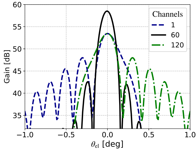
Fig. 15. Antenna pattern defocusing effects on gain and beamwidth for the center and edge channels in elevation (created using GRASP software).
