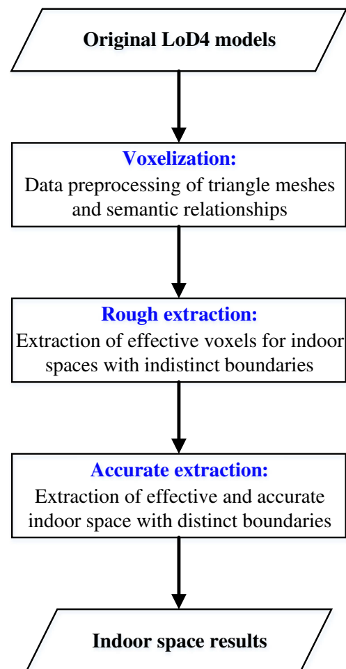
Fig. 5 Flowchart of the proposed automated indoor space extraction algorithm
