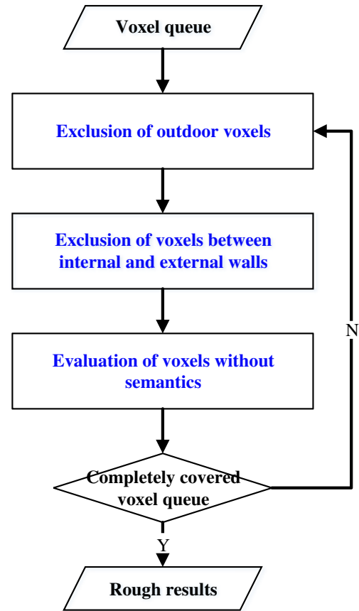
Fig. 9 Flowchart of rough extraction
