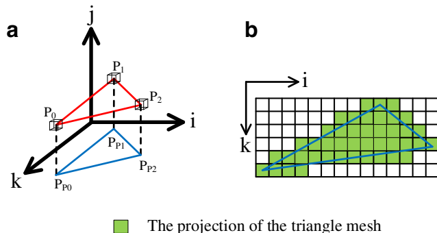
Fig. 8 Voxelization of the triangular mesh
