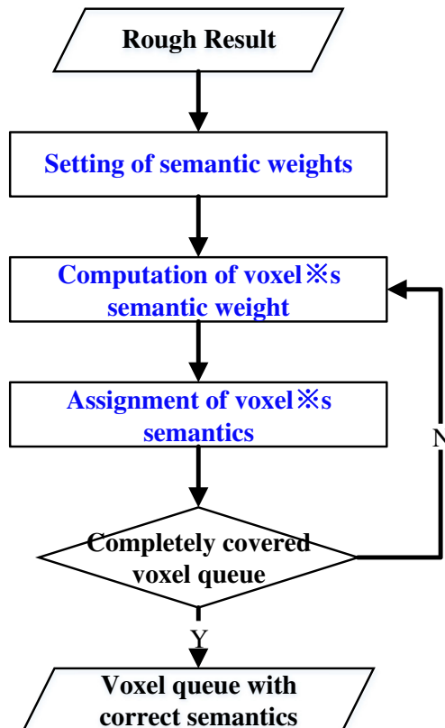
Fig. 11 Flowchart of the update procedure for the voxels' semantics
