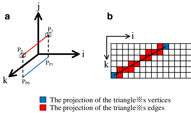
Fig. 7 Voxelization of an edge
