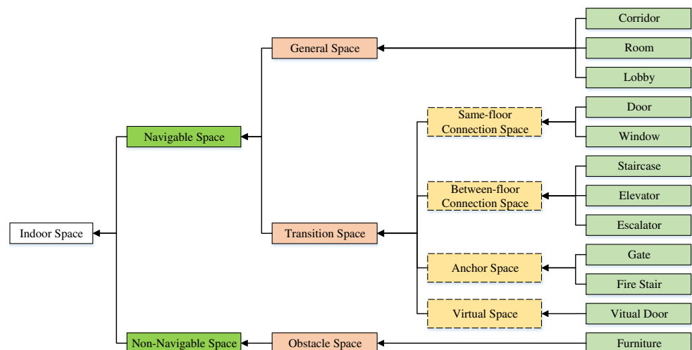
Fig. 4 Hierarchy of semantic information for indoor spaces
