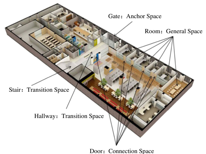
Fig. 2 Classification of indoor spaces in IndoorGML
