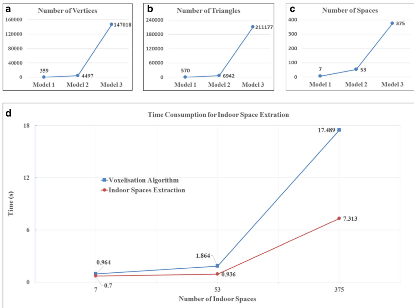
Fig. 16 Experimental statistics
