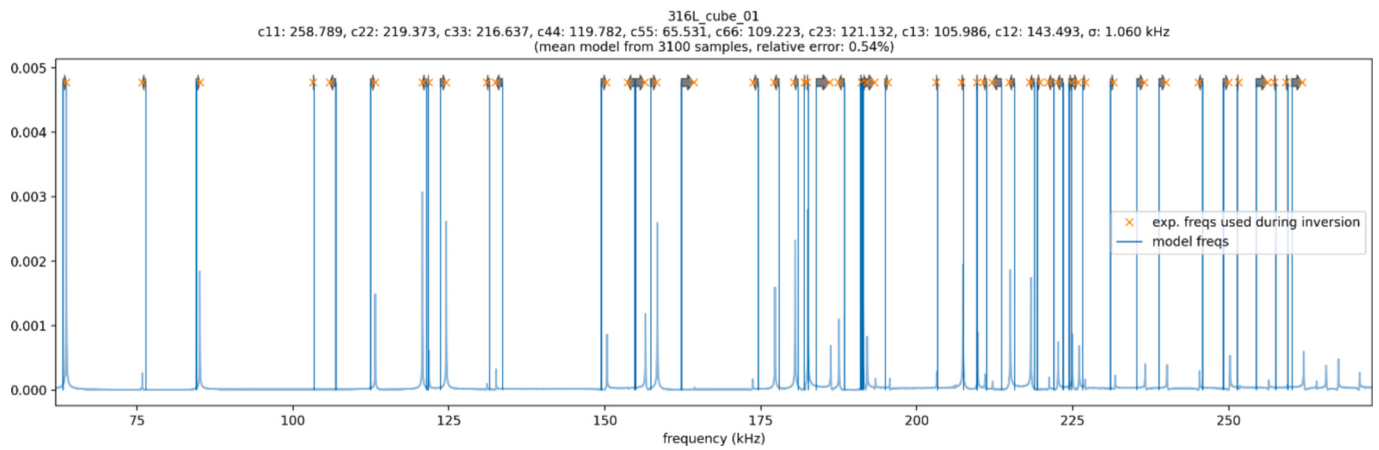
Fig. 7. Effective orthotropic RUS inversion result for 316 L sample 1. The measured spectrum is shown along with extracted peaks as crosses, and the fitted model shown as vertical bars.
