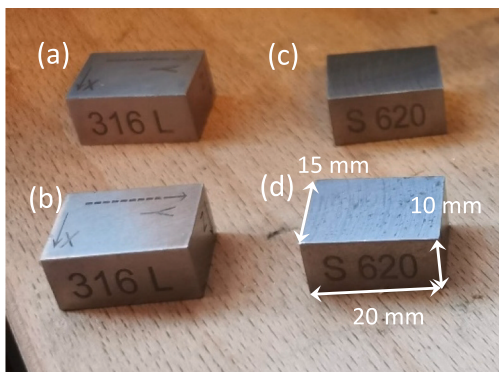
Fig. 1. (left) Metallic samples analysed in this study: austenitic 316 L samples (a) and (b), S620 samples (c) and (d). (right) Schematic depiction of S620 samples original location within massive block with block reference frame (identical to sample reference frame).
