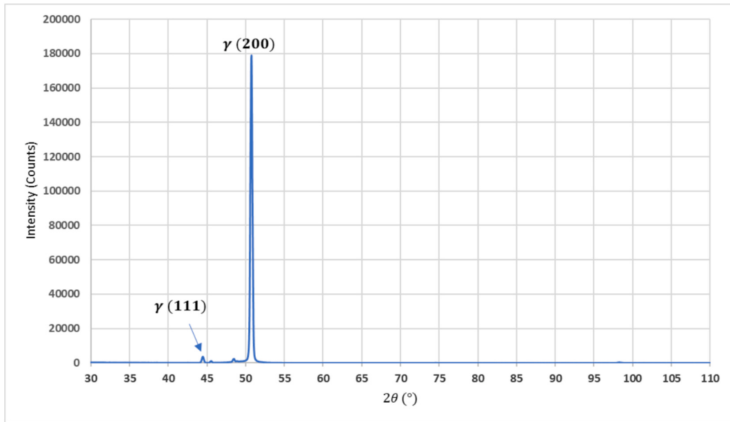
Fig. 2. XRD pattern of one of the WAAM processed 316 L stainless steel, showing intensity of selected austenite peaks.
