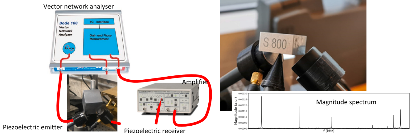
Fig. 3. Experimental setup used for resonance frequency measurement and example magnitude spectrum.
