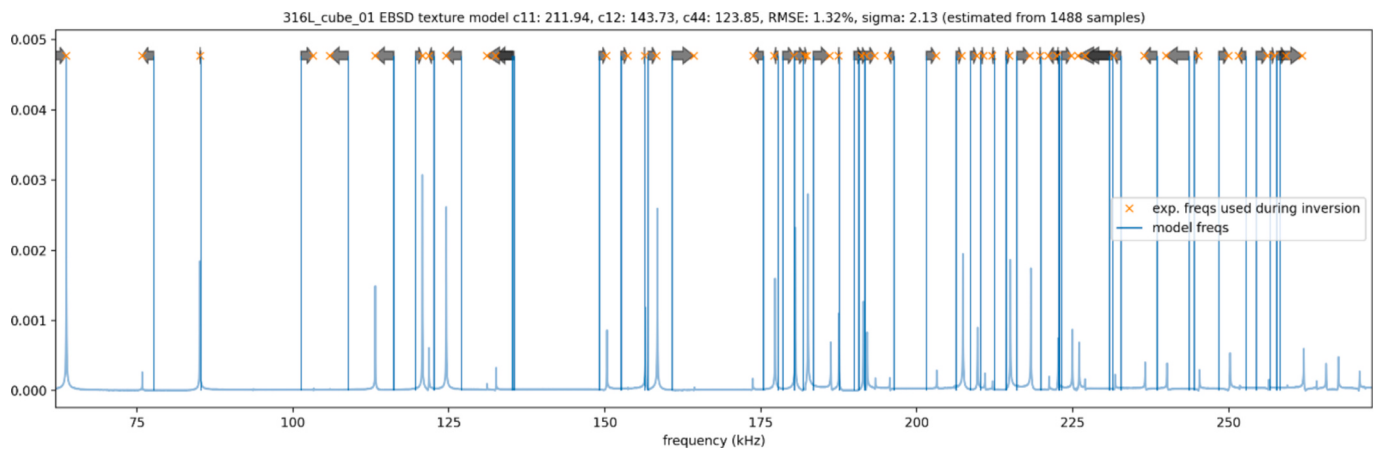
Fig. 8. EBSD texture-based elastic model inversion result for 316 L sample 1. The measured spectrum is shown along with extracted peaks as crosses, and the fitted model shown as vertical bars.
