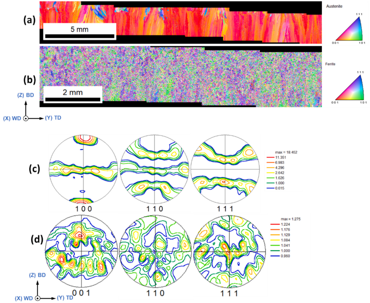
Fig. 5. (a) and (b): BD-IPF maps of 316 L and S620 steels respectively, (c) and (d) The pole figures of 316 L and S620 steels, respectively.
