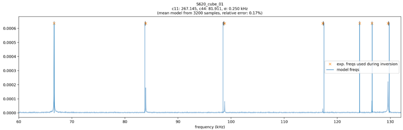
Fig. 6. RUS inversion result for S620 sample 1. The measured spectrum is shown along with extracted peaks as crosses, and the fitted model shown as vertical bars.
