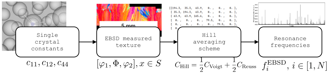
Fig. 4. Schematic description of the model based on measured texture and single crystal elastic constants.
