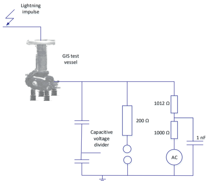
Figure 5-12: Circuit diagram for breakdown under superposed voltage stresses in GIS due to protrusions
