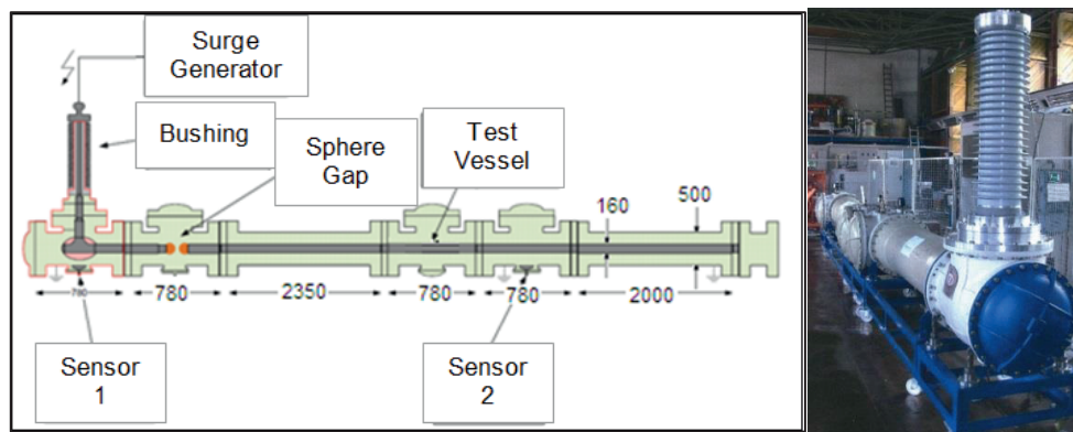
Figure 5-6: VFTO test setup (550-kV GIS) in the laboratory of Stuttgart University of Technology
