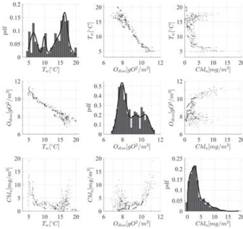
Fig. 2. Overview of sampled data for mussel cultivation case: daily maximum T_w and concomitants for minimum O_{diss} and Chla . The univariate histograms with fitted pdfs are displayed on the diagonal
