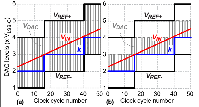
Fig. 2: SAR output ( k ) and \Delta\Sigma DAC swings with M = 1 for (a) a 1b quantizer and (b) a 2b quantizer
