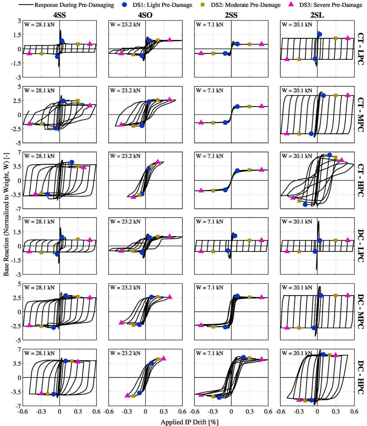
Fig. 12. Load-displacement response of different specimens during IP pre-damaging. The response of each specimen is normalized to its weight, W , for easier comparison. W is the weight of each specimen excluding the top beam and the base, and is 28.08 kN for 4SS, 23.16 kN for 4SO, 7.1 kN for 2SS, and 20.1 kN for 2SL.
