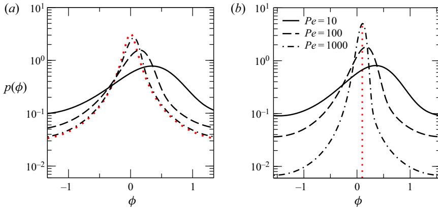
Figure 6. Steady-state orientation distribution function p(\phi) for a real ( k_e = 0.1 ) or a purely imaginary ( k_e = 0.1i ) value of k_e for different Pe numbers. The red dotted line marks the orientation distribution function for Pe \rightarrow \infty and k_e = 0.1 (a) and the location of \phi_c for k_e = 0.1i (b). The values [\mu, \sigma^2, \langle(\phi - \mu)^3\rangle] in increasing order of Pe are [0.17, 0.39, -0.36] , [0.069, 0.21, -0.40] and [0.019, 0.14, -0.30] , respectively, for k_e = 0.1 ; and [0.19, 0.38, -0.37] , [0.094, 0.16, -0.53] and [0.075, 0.033, -1.1] , respectively, for k_e = 0.1i .
