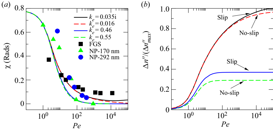
Figure 17. Comparison of our theory (for \theta = \pi/2 ) with experimental results of Reddy et al. (2018) for \chi and \Delta n''/\Delta n''_{max} (symbols), as defined in (5.1a,b). The different lines correspond to the following model parameters: functionalised graphene platelets (FGS) with k_e \approx 0.016 (no-slip) and k_e = 0.035i (slip with \lambda = 20 nm); slightly oblate nanospheroids (NP) with b/a = 0.55 , for k_e \approx 0.55 (no-slip) and k_e \approx 0.46 (slip with \lambda/b = 0.21 ).
