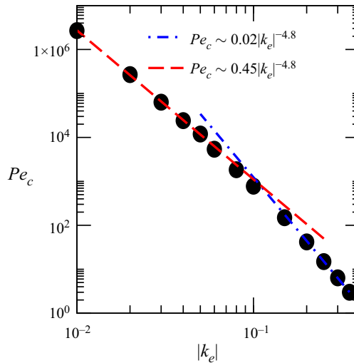
Figure 8. Threshold value of the Péclet number Pe_c beyond which no platelet rotation is expected, as a function of |k_e| (with k_e purely imaginary). Black disks are numerical values, lines are fits for |k_e| \gtrsim 0.1 (dot-dashed blue line) and |k_e| \lesssim 0.1 (dashed red line), respectively.
