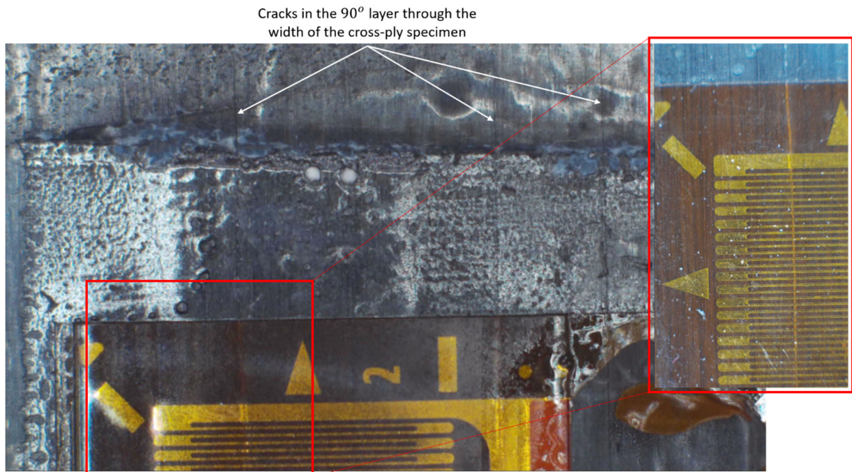
Figure 9. Local failure of the 90^\circ layer for the cross-ply configuration.
