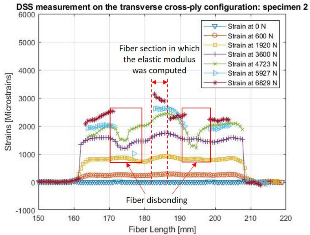
Figure 8. DSS strain measurements for specimen 2 of the transverse cross-ply configuration.
