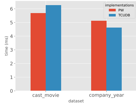
Fig. 10: Execution time tested on real-world datasets.
