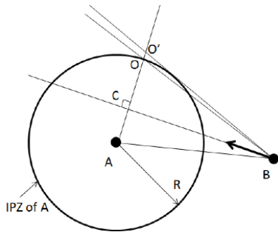
Figure 2: Finding the displacement vector in MVP
