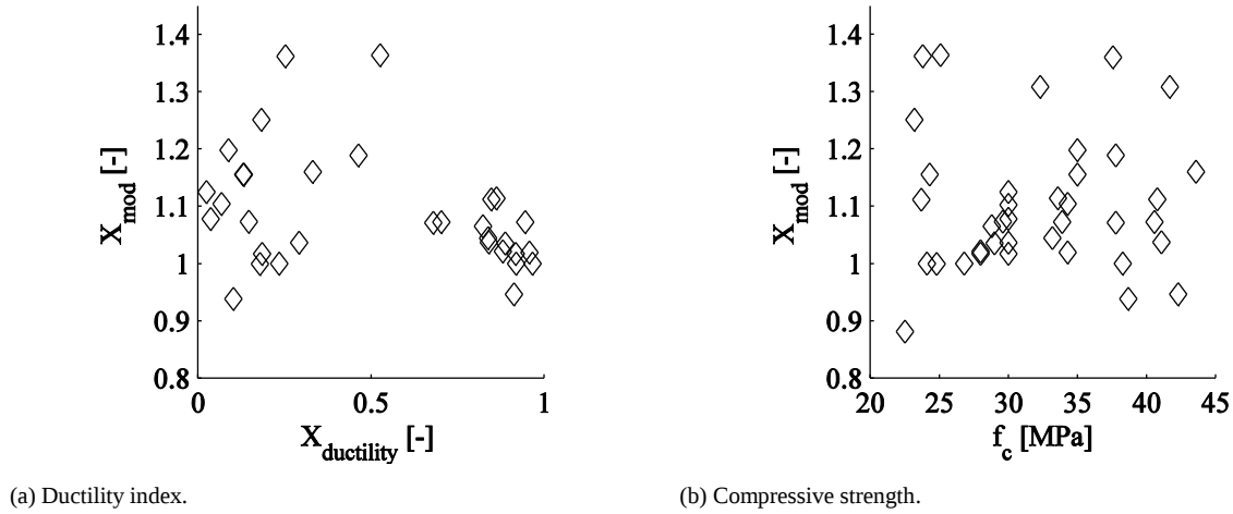
Fig. 4. Correlation between modelling uncertainty X_{\text{mod}} and a) ductility index X_{\text{ductility}} and b) compressive strength f_c .
