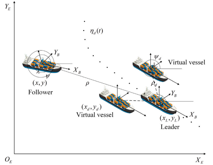
Fig. 1. The formation structure of the leader-follower approach.
