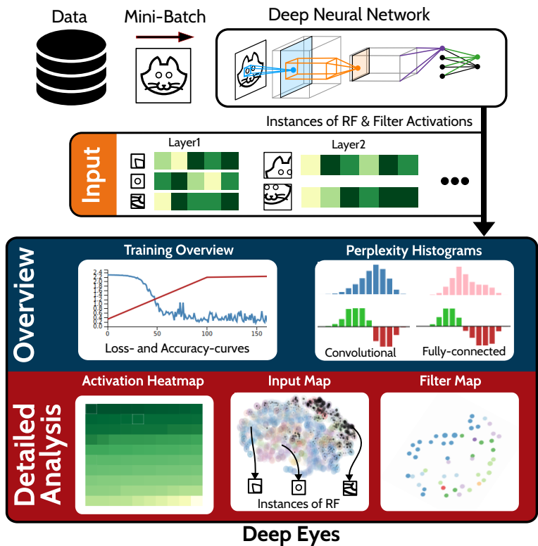
Figure 9.5: Overview of the DeepEyes system. The network training overview provided by the loss- and accuracy-curves is integrated with the Perplexity Histograms that allow for the identification of stable layers in the network (blue background). The user focuses on stable layers that are analyzed in detail with three tightly linked visualizations, namely the Activation Heatmap, the Input Map and the Filter Map (red background).
