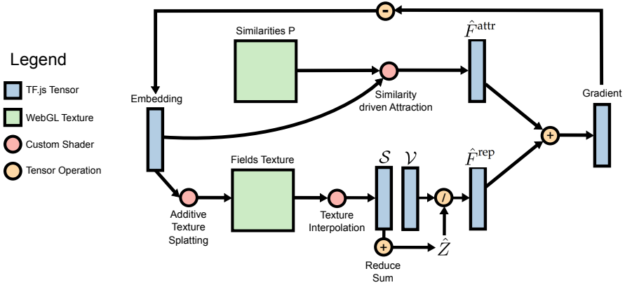
Figure 5.3: Computational workflow of our approach. On the lower side the of the chart, the computation of the repulsive forces is presented. The fields texture is generated by the additive texture splatting presented in Section 5.3.2. The value of \mathcal{S} and \mathcal{V} are obtained through a texture interpolation and are used to compute the repulsive forces. The attractive forces are computed in a custom WebGL shader that takes as input the similarities P and the embedding. The gradient of the objective function is then computed and used to update the embedding.
