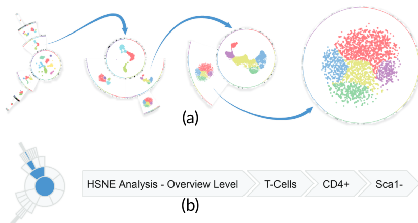
Figure 7.3: Adaptive layout of CyteGuide. Detailed embeddings can be placed at the center to reduce clutter (a). A thumbnail and breadcrumb visualization is used to keep track of the interaction (b).
