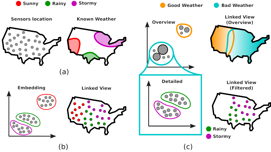
Figure 6.5: Traditional vs Hierarchical analysis. (a) High-dimensional readings from sensors located on a map and prior knowledge on the phenomenon of interest are available to the user. In the traditional analysis (b) a single embedding is generated and analyzed. In our hierarchical analysis (c), an overview shows dominant structures in the dataset. Detailed embedding of the structures are created by filtering and drilling into the data.
