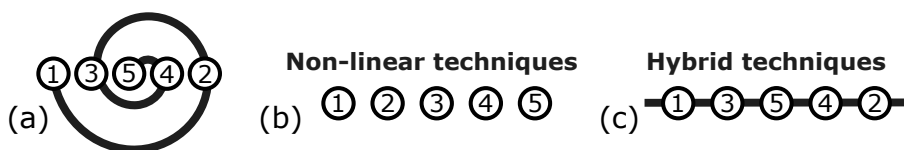
Figure 6.1: Dimensionality reduction with landmarks. In non-linear embedding techniques the underlying manifold (a) is respected (b). In hybrid approaches, landmarks are placed without considering the underlying manifold (c) and data points are placed by interpolating the landmark positions (grey line in c). The layout quality thus relates to the used number of landmarks.
