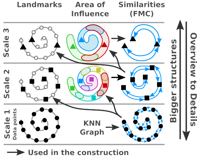
Figure 6.2: Overview of the hierarchy construction. A Finite Markov Chain (FMC) is built from the k-nearest neighbor graph. The FMC encodes the similarities between landmarks and it is used for selecting landmarks in the next scale. The FMC is also used to compute the area of influence of the selected landmarks on the landmarks in the lower scale. The overlap between the areas of influence is used to build a new FMC that encodes similarities in the new scale.
