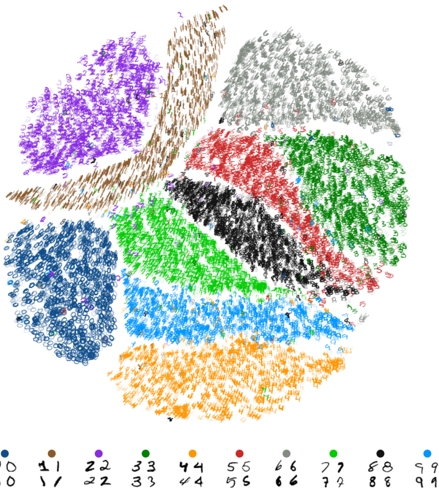
Figure 3.2: tSNE embedding of the MNIST dataset. The embedded data points are visualized as the MNIST images colored according to the digit they represent. Ten manifolds, one for each digit, are visible.
