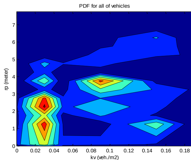
Figure 4 Distribution of pore space ( r_p ) and density ( k_v ) for interaction between vehicles on the cross-section road without specific lane
