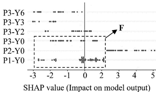
FIGURE 14 SHAP plot for different “Phases-Year” in fatigue resistance model (For acronyms, refer to Table 2).
