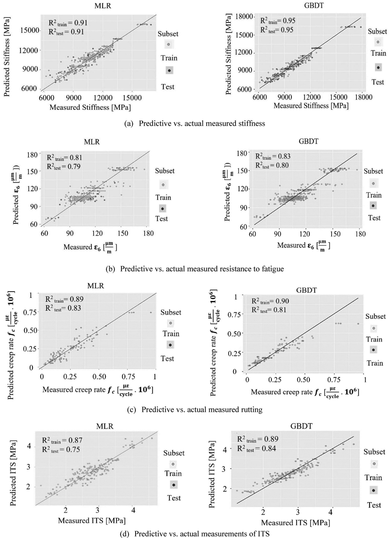
FIGURE 4 Performance comparison of gradient boosting decision tree (GBDT) and multilinear regression (MLR) models. (a) Predictive versus actual measured stiffness; (b) predictive versus actual measured resistance to fatigue, (c) predictive versus actual measured rutting, and (d) predictive versus actual measurements of ITS.
