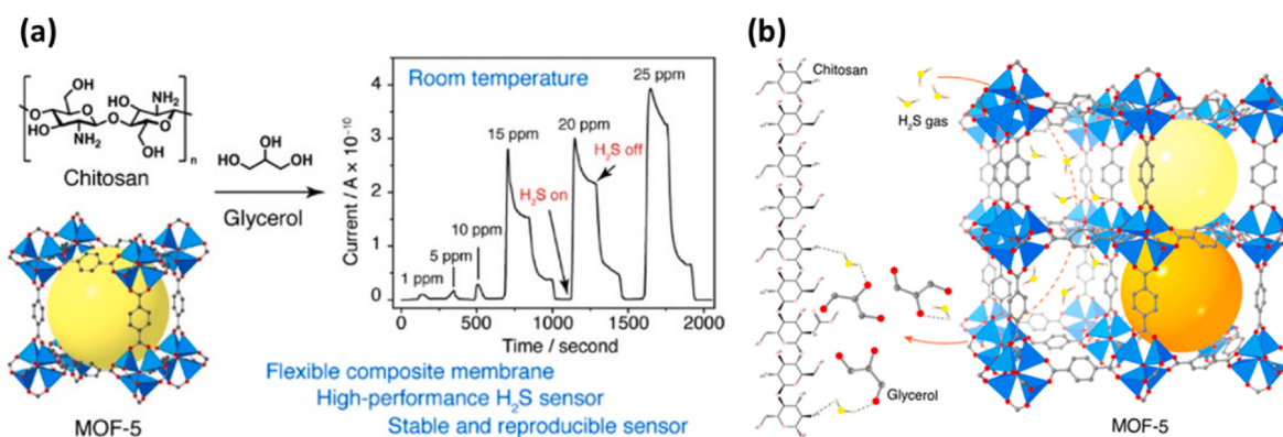
Fig. 9. (a) Electrical current signal of Ch-IL-MOF composite sensor as a function of \text{H}_2\text{S} concentration and time; (b) Pictorial representation of proposed \text{H}_2\text{S} gas-sensing mechanism. Atom colors: S, yellow; Zn, aqua; O, red; N, blue; C, grey; and H, pastel red. Reprinted with permission from (A. Ali et al., 2021). (For interpretation of the references to colour in this figure legend, the reader is referred to the Web version of this article.)
