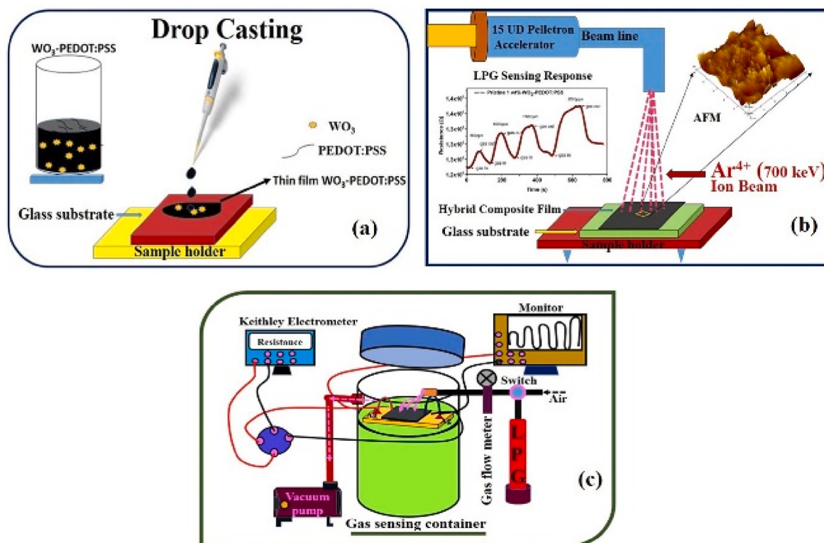
Fig. 11. (a) Schematic illustration of preparing nanohybrid thin films on glass substrate via drop casting technique; (b) Pictorial diagram of \text{Ar}^{4+} ion beam (700 keV) irradiation of hybrid nanohybrid film; and (c) The schematic demonstration of gas sensing setup. Reprinted with permission from (Ram et al., 2020).
