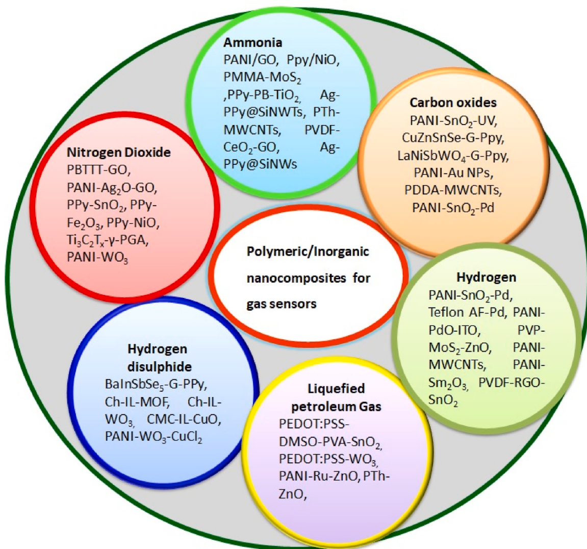
Fig. 3. Gas sensing applications of various polymeric/inorganic nanohybrids.
