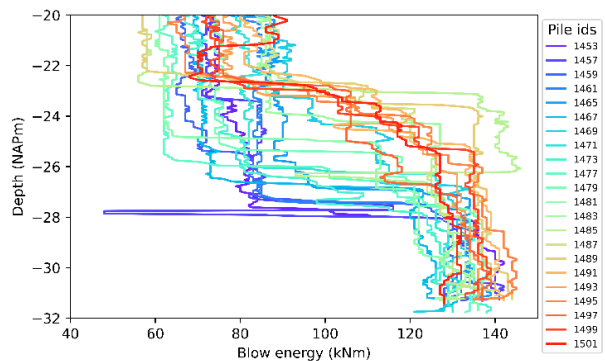
Figure 8. Drive energy.
